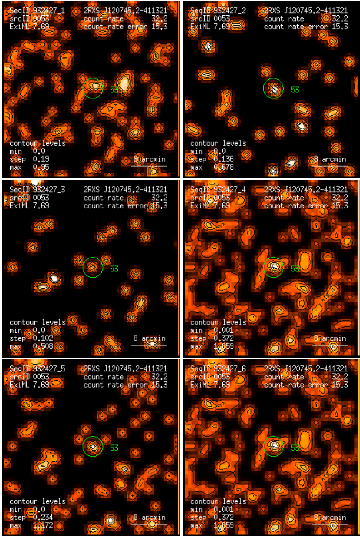
Figure 53: RASS 932427: detection 0053: band rate images, Gaussian filter: (1) PSPC channels 11 – 41, (2) 52 – 90, (3) 91 – 201, (4) 11 – 235, (5) 52 – 201, (6) 11 – 201. Broad band rates in counts/ks. Band rate contour levels in counts/ks/arcmin 2 .
