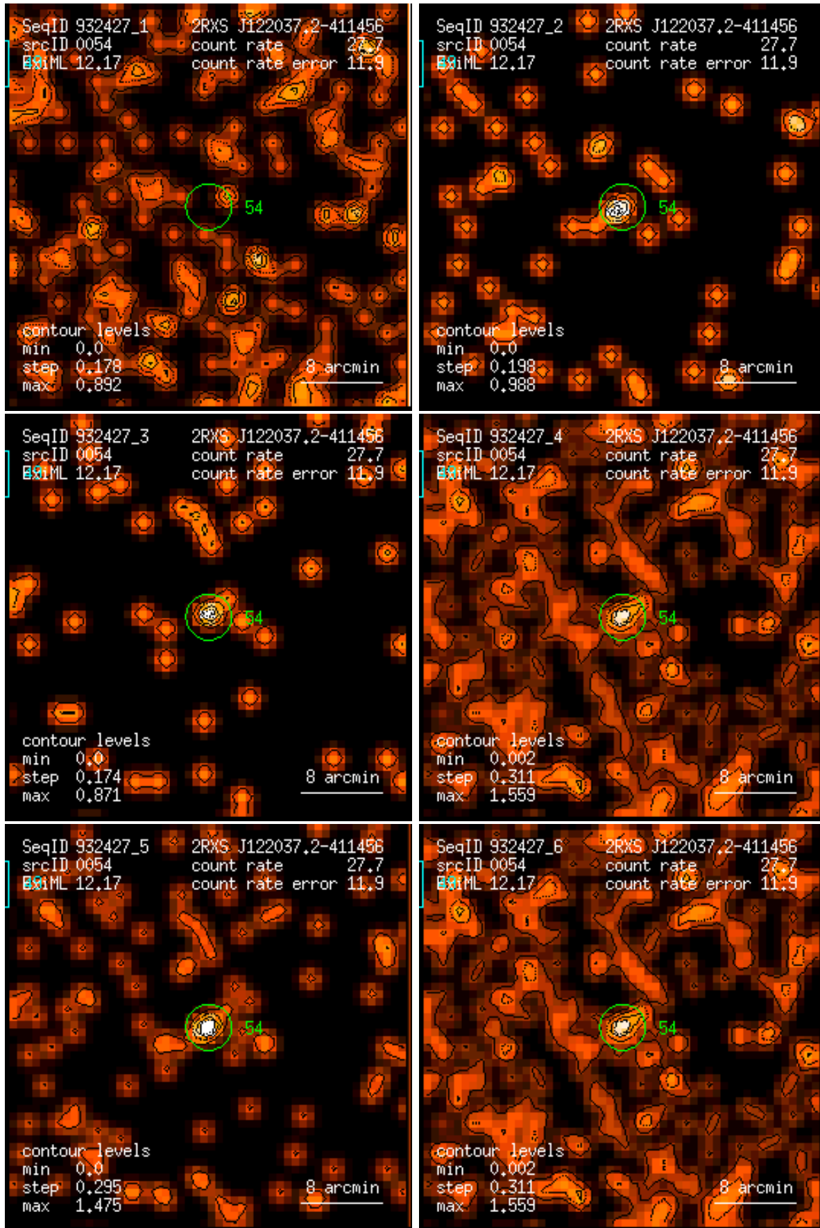
Figure 54: RASS 932427: detection 0054: band rate images, Gaussian filter: (1) PSPC channels 11 – 41, (2) 52 – 90, (3) 91 – 201, (4) 11 – 235, (5) 52 – 201, (6) 11 – 201. Broad band rates in counts/ks. Band rate contour levels in counts/ks/arcmin 2 .
