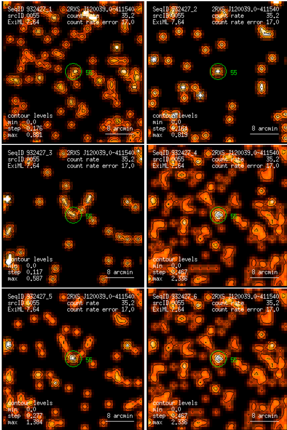
Figure 55: RASS 932427: detection 0055: band rate images, Gaussian filter: (1) PSPC channels 11 – 41, (2) 52 – 90, (3) 91 – 201, (4) 11 – 235, (5) 52 – 201, (6) 11 – 201. Broad band rates in counts/ks. Band rate contour levels in counts/ks/arcmin 2 .
