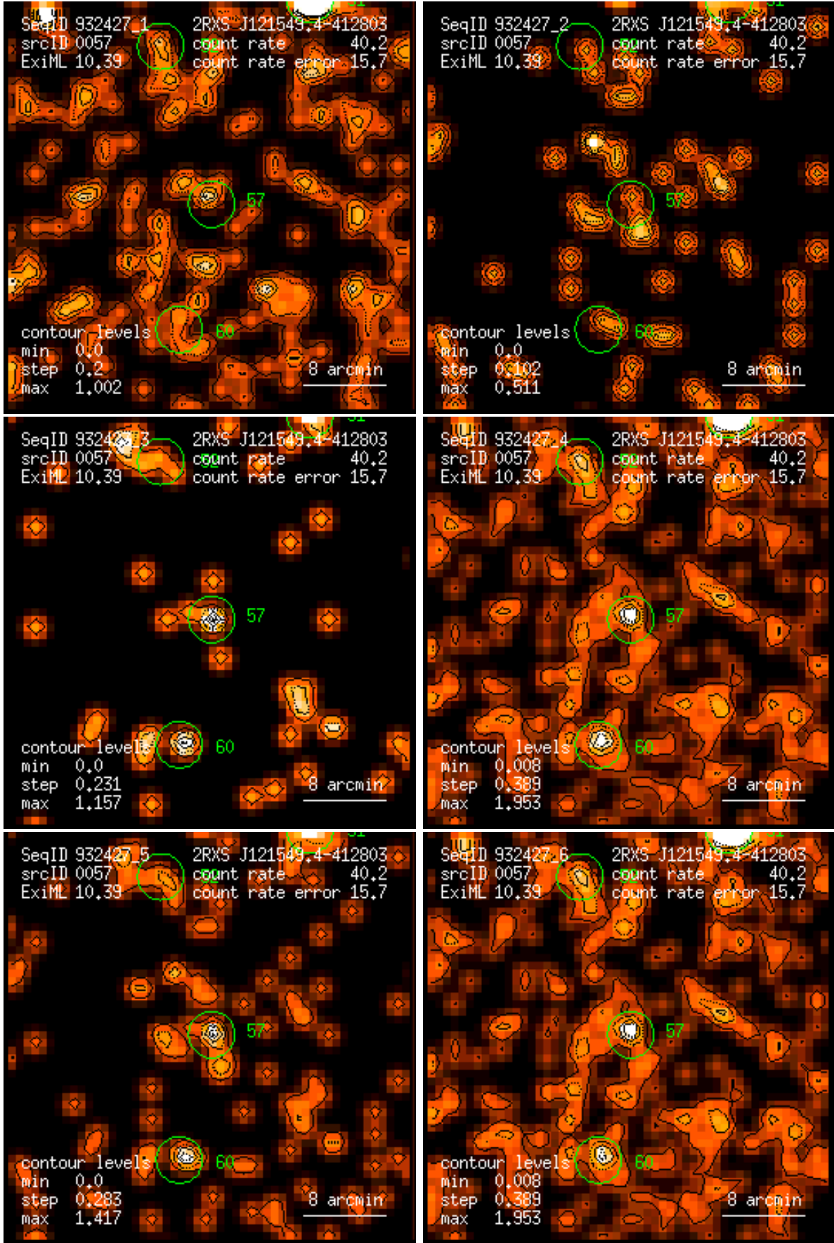
Figure 57: RASS 932427: detection 0057: band rate images, Gaussian filter: (1) PSPC channels 11 – 41, (2) 52 – 90, (3) 91 – 201, (4) 11 – 235, (5) 52 – 201, (6) 11 – 201. Broad band rates in counts/ks. Band rate contour levels in counts/ks/arcmin 2 .
