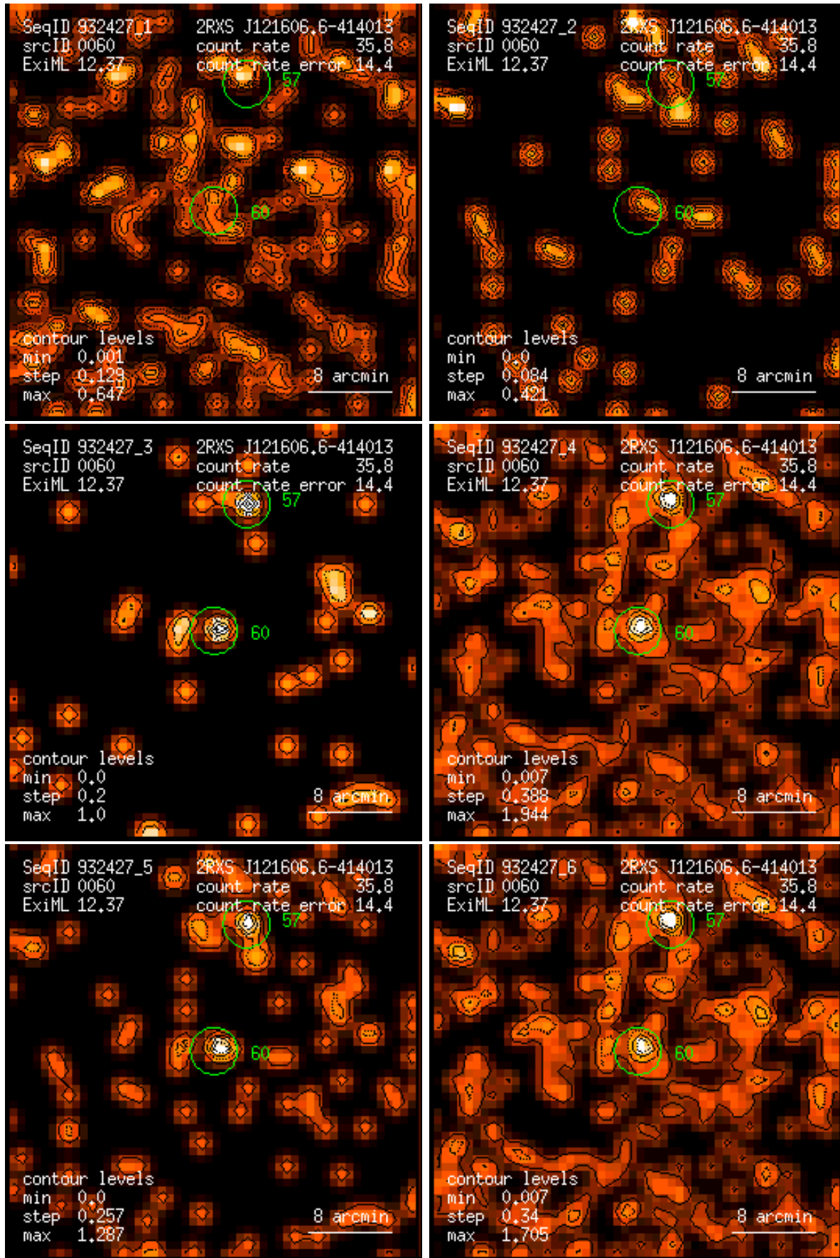
Figure 60: RASS 932427: detection 0060: band rate images, Gaussian filter: (1) PSPC channels 11 – 41, (2) 52 – 90, (3) 91 – 201, (4) 11 – 235, (5) 52 – 201, (6) 11 – 201. Broad band rates in counts/ks. Band rate contour levels in counts/ks/arcmin 2 .
