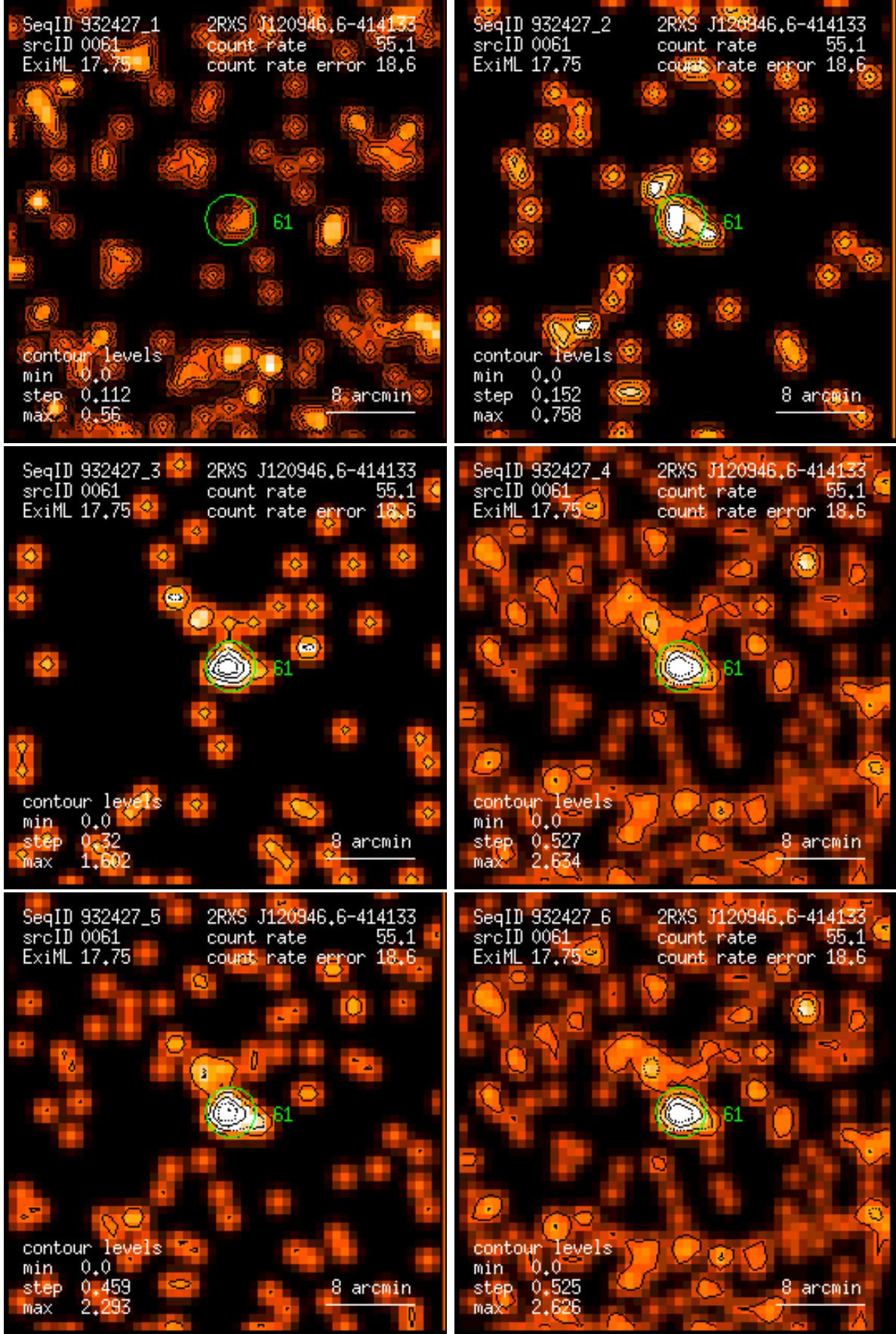
Figure 61: RASS 932427: detection 0061: band rate images, Gaussian filter: (1) PSPC channels 11 – 41, (2) 52 – 90, (3) 91 – 201, (4) 11 – 235, (5) 52 – 201, (6) 11 – 201. Broad band rates in counts/ks. Band rate contour levels in counts/ks/arcmin 2 .
