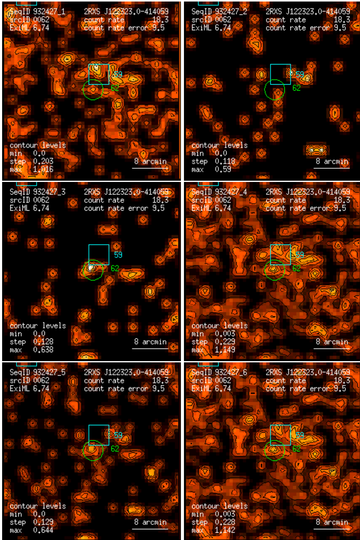
Figure 62: RASS 932427: detection 0062: band rate images, Gaussian filter: (1) PSPC channels 11 – 41, (2) 52 – 90, (3) 91 – 201, (4) 11 – 235, (5) 52 – 201, (6) 11 – 201. Broad band rates in counts/ks. Band rate contour levels in counts/ks/arcmin 2 .
