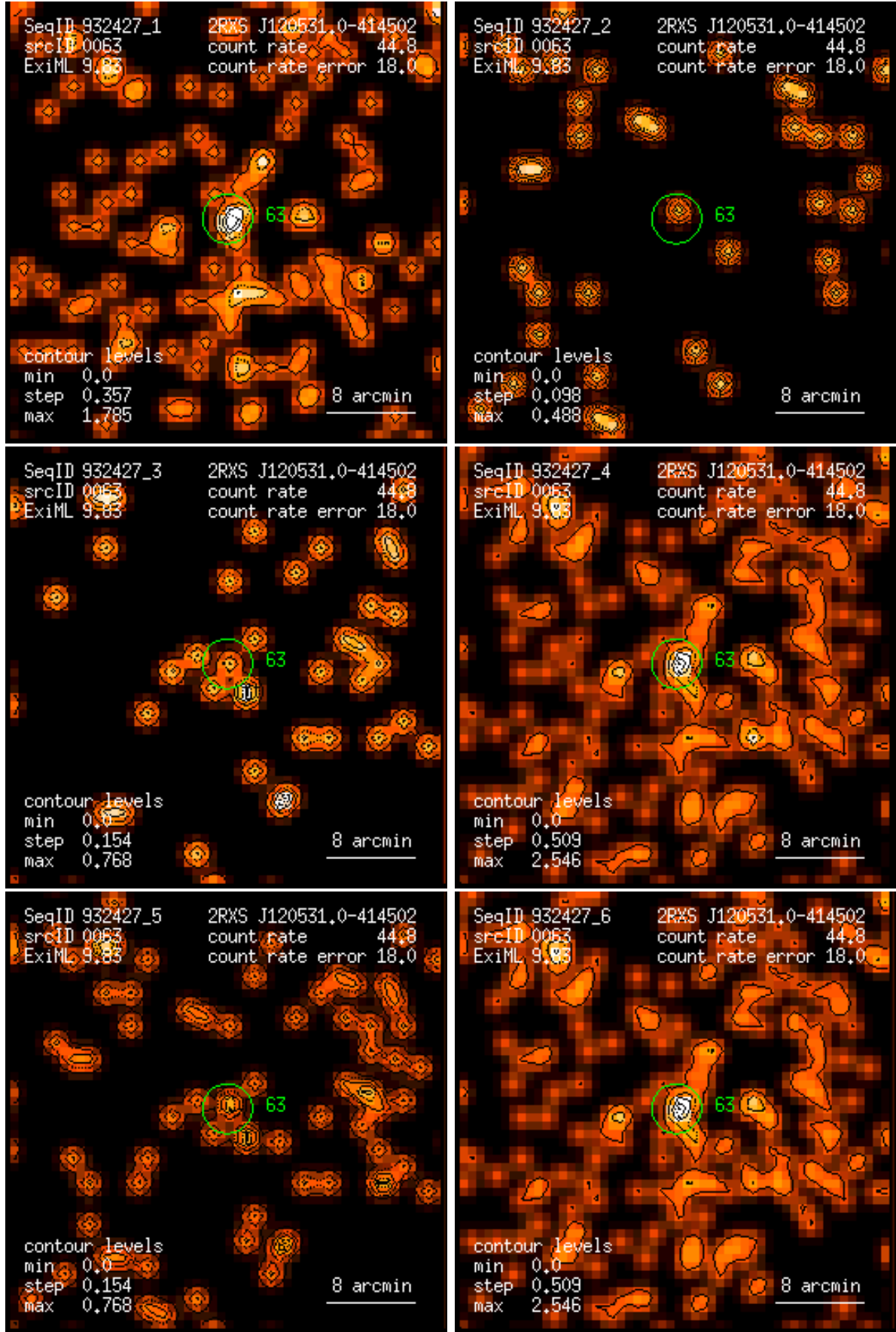
Figure 63: RASS 932427: detection 0063: band rate images, Gaussian filter: (1) PSPC channels 11 – 41, (2) 52 – 90, (3) 91 – 201, (4) 11 – 235, (5) 52 – 201, (6) 11 – 201. Broad band rates in counts/ks. Band rate contour levels in counts/ks/arcmin 2 .
