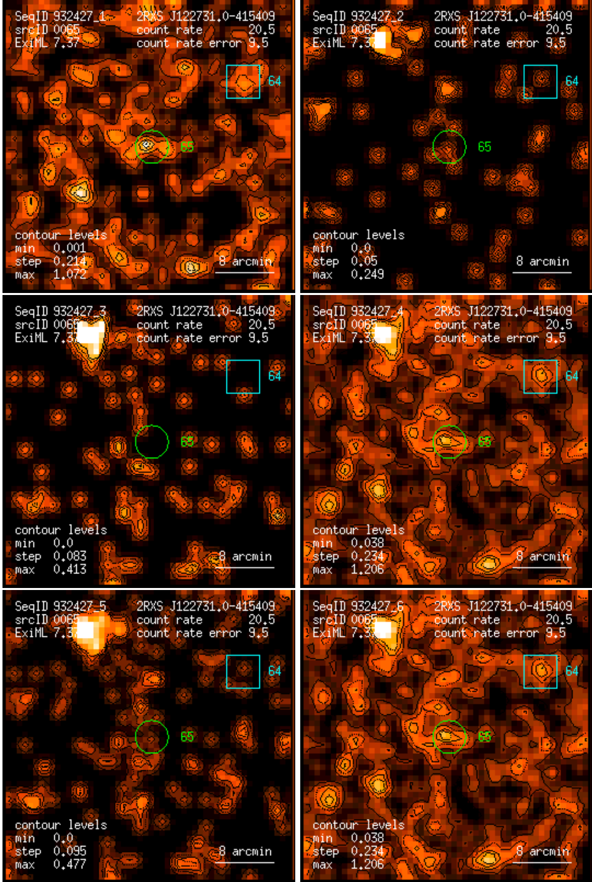
Figure 65: RASS 932427: detection 0065: band rate images, Gaussian filter: (1) PSPC channels 11 – 41, (2) 52 – 90, (3) 91 – 201, (4) 11 – 235, (5) 52 – 201, (6) 11 – 201. Broad band rates in counts/ks. Band rate contour levels in counts/ks/arcmin 2 .
