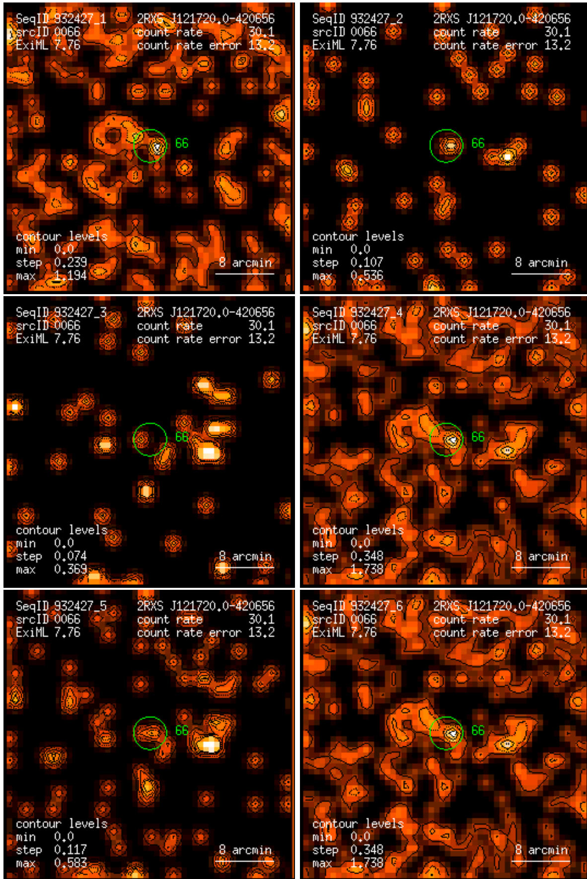
Figure 66: RASS 932427: detection 0066: band rate images, Gaussian filter: (1) PSPC channels 11 – 41, (2) 52 – 90, (3) 91 – 201, (4) 11 – 235, (5) 52 – 201, (6) 11 – 201. Broad band rates in counts/ks. Band rate contour levels in counts/ks/arcmin 2 .
