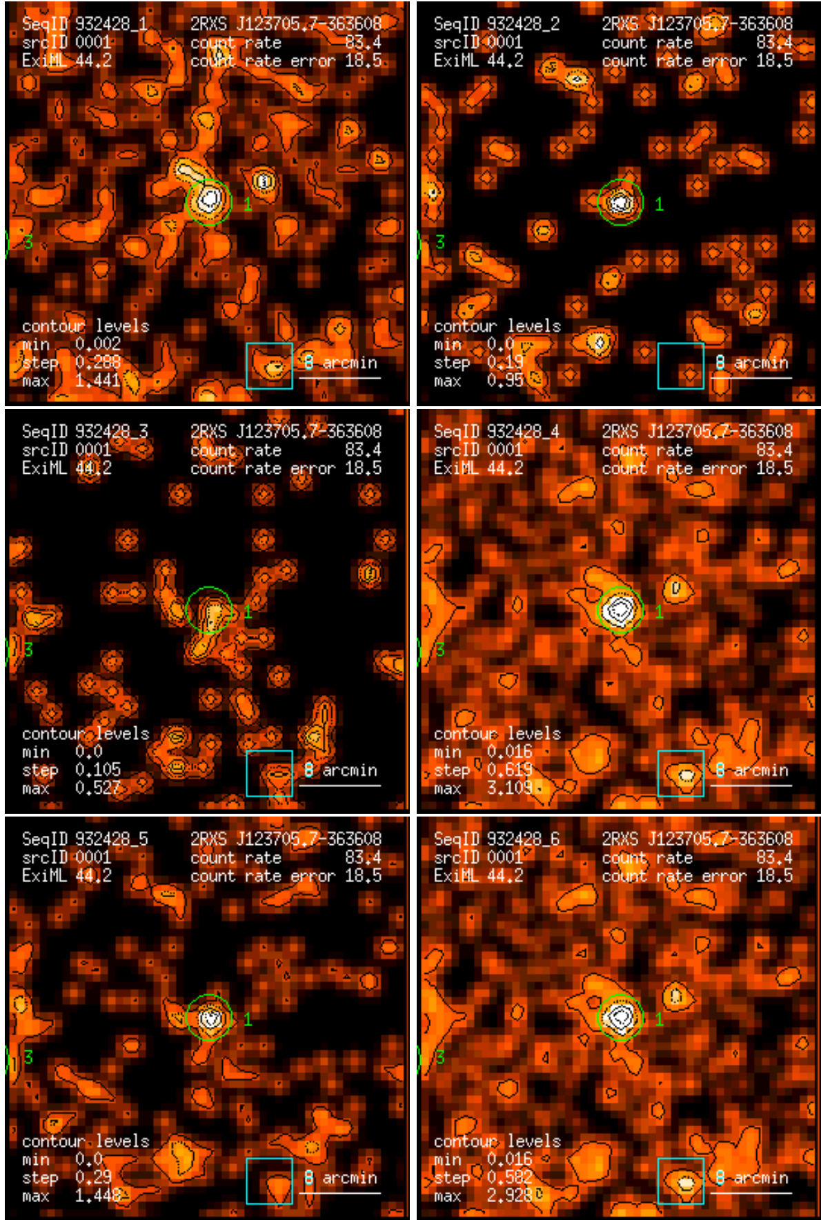
Figure 1: RASS 932428: detection 0001: band rate images, Gaussian filter: (1) PSPC channels 11 – 41, (2) 52 – 90, (3) 91 – 201, (4) 11 – 235, (5) 52 – 201, (6) 11 – 201. Broad band rates in counts/ks. Band rate contour levels in counts/ks/arcmin 2 .
