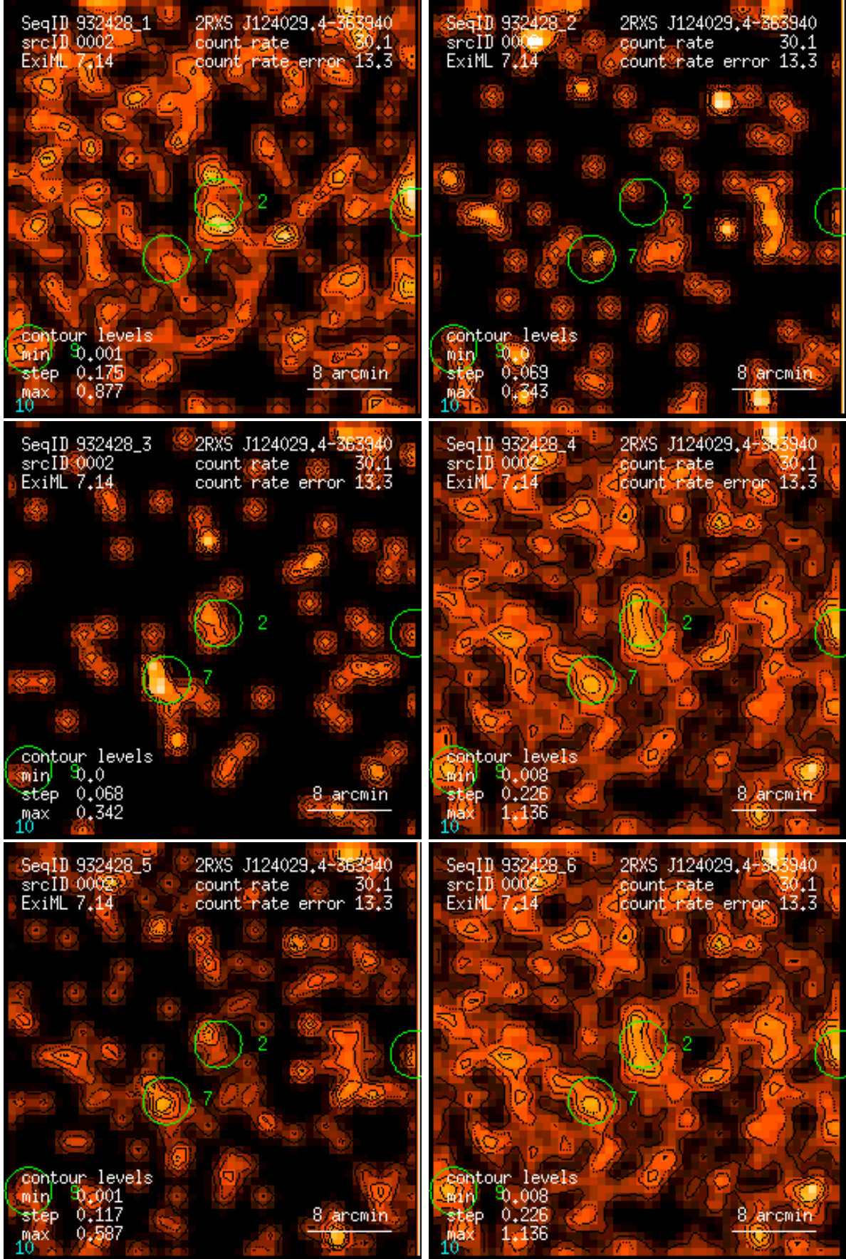
Figure 2: RASS 932428: detection 0002: band rate images, Gaussian filter: (1) PSPC channels 11 – 41, (2) 52 – 90, (3) 91 – 201, (4) 11 – 235, (5) 52 – 201, (6) 11 – 201. Broad band rates in counts/ks. Band rate contour levels in counts/ks/arcmin 2 .
