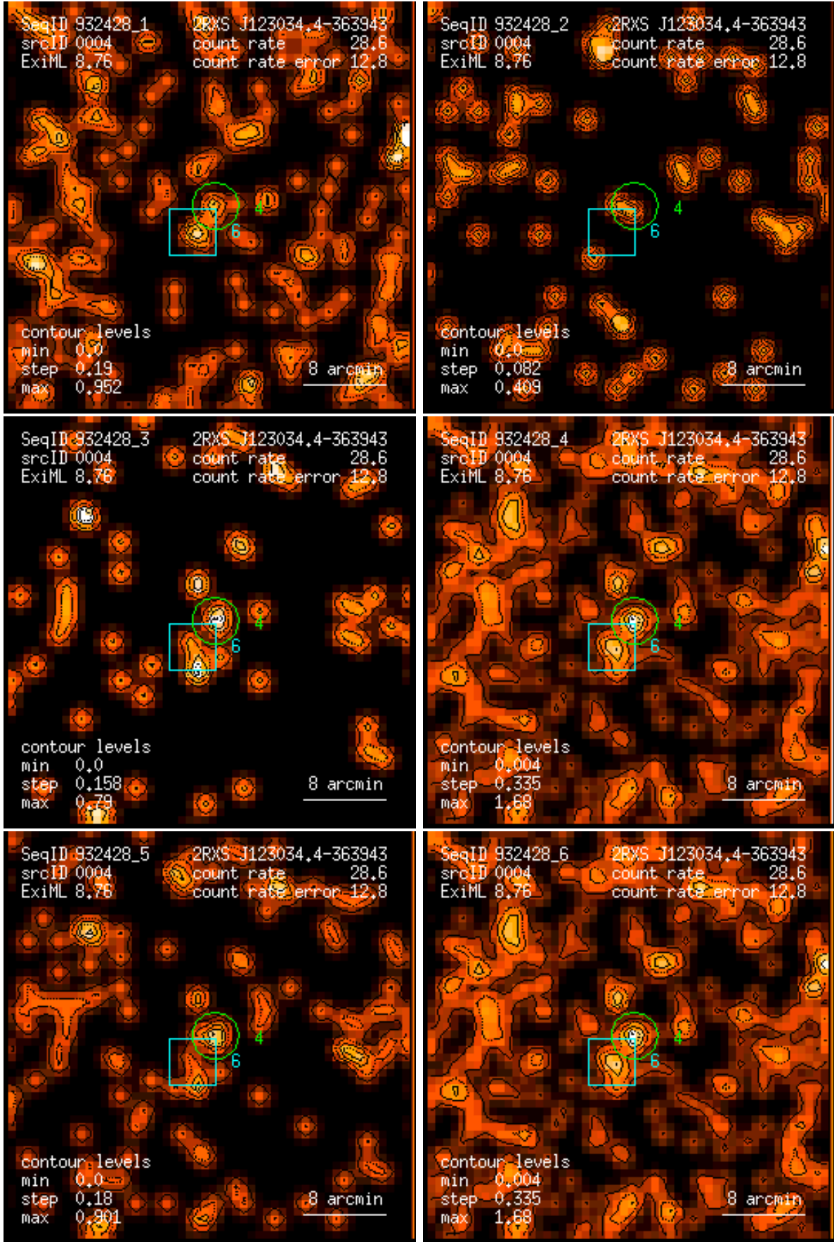
Figure 4: RASS 932428: detection 0004: band rate images, Gaussian filter: (1) PSPC channels 11 – 41, (2) 52 – 90, (3) 91 – 201, (4) 11 – 235, (5) 52 – 201, (6) 11 – 201. Broad band rates in counts/ks. Band rate contour levels in counts/ks/arcmin 2 .
