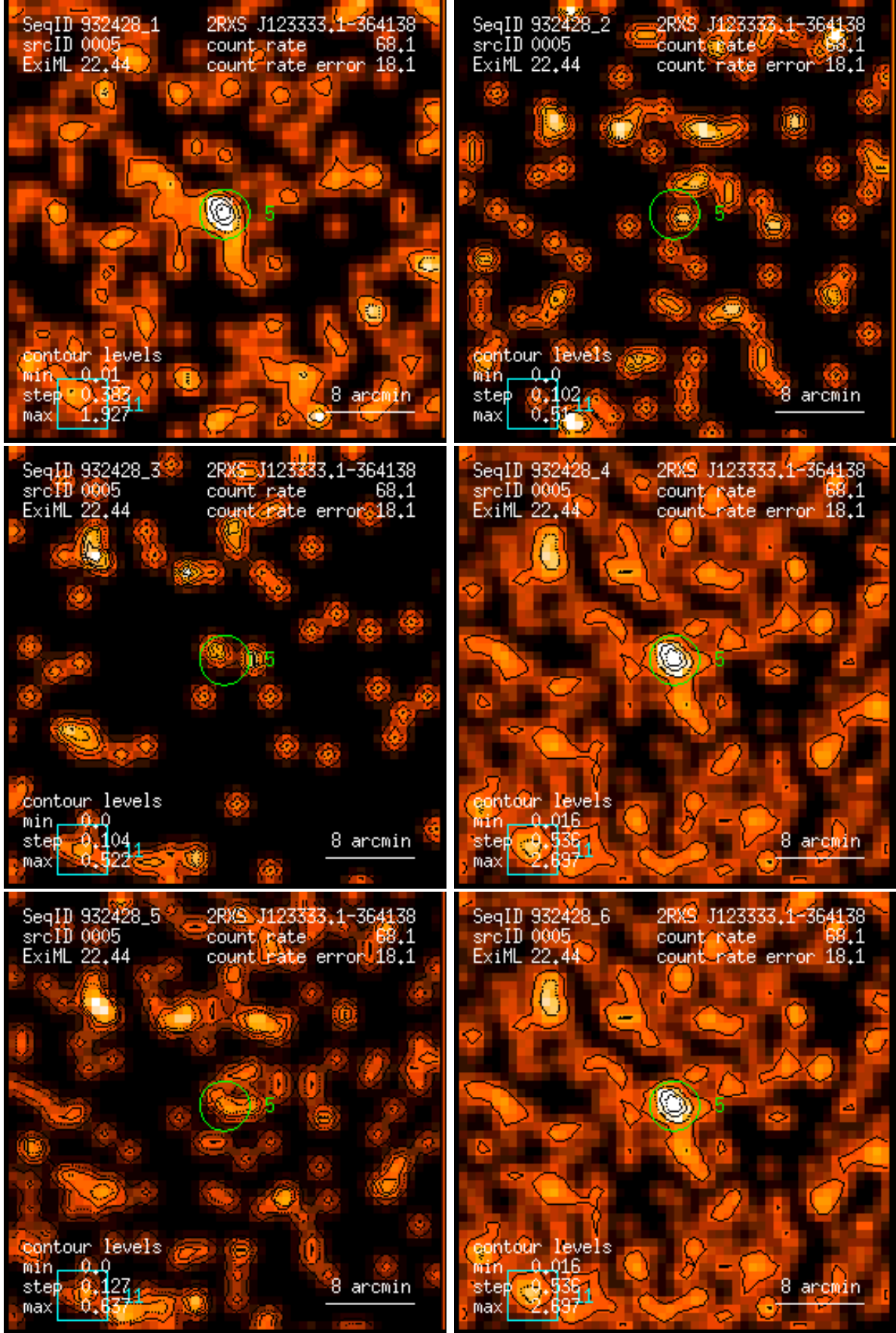
Figure 5: RASS 932428: detection 0005: band rate images, Gaussian filter: (1) PSPC channels 11 – 41, (2) 52 – 90, (3) 91 – 201, (4) 11 – 235, (5) 52 – 201, (6) 11 – 201. Broad band rates in counts/ks. Band rate contour levels in counts/ks/arcmin 2 .
