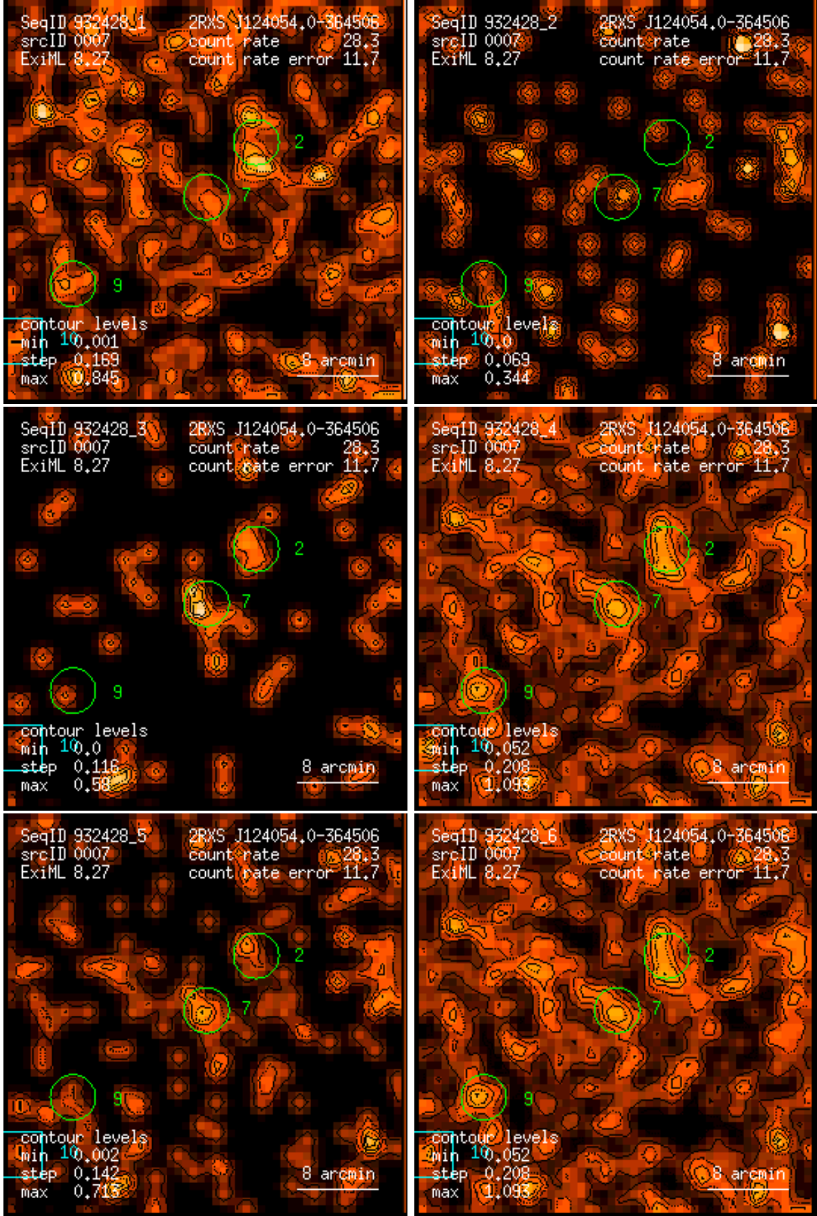
Figure 7: RASS 932428: detection 0007: band rate images, Gaussian filter: (1) PSPC channels 11 – 41, (2) 52 – 90, (3) 91 – 201, (4) 11 – 235, (5) 52 – 201, (6) 11 – 201. Broad band rates in counts/ks. Band rate contour levels in counts/ks/arcmin 2 .
