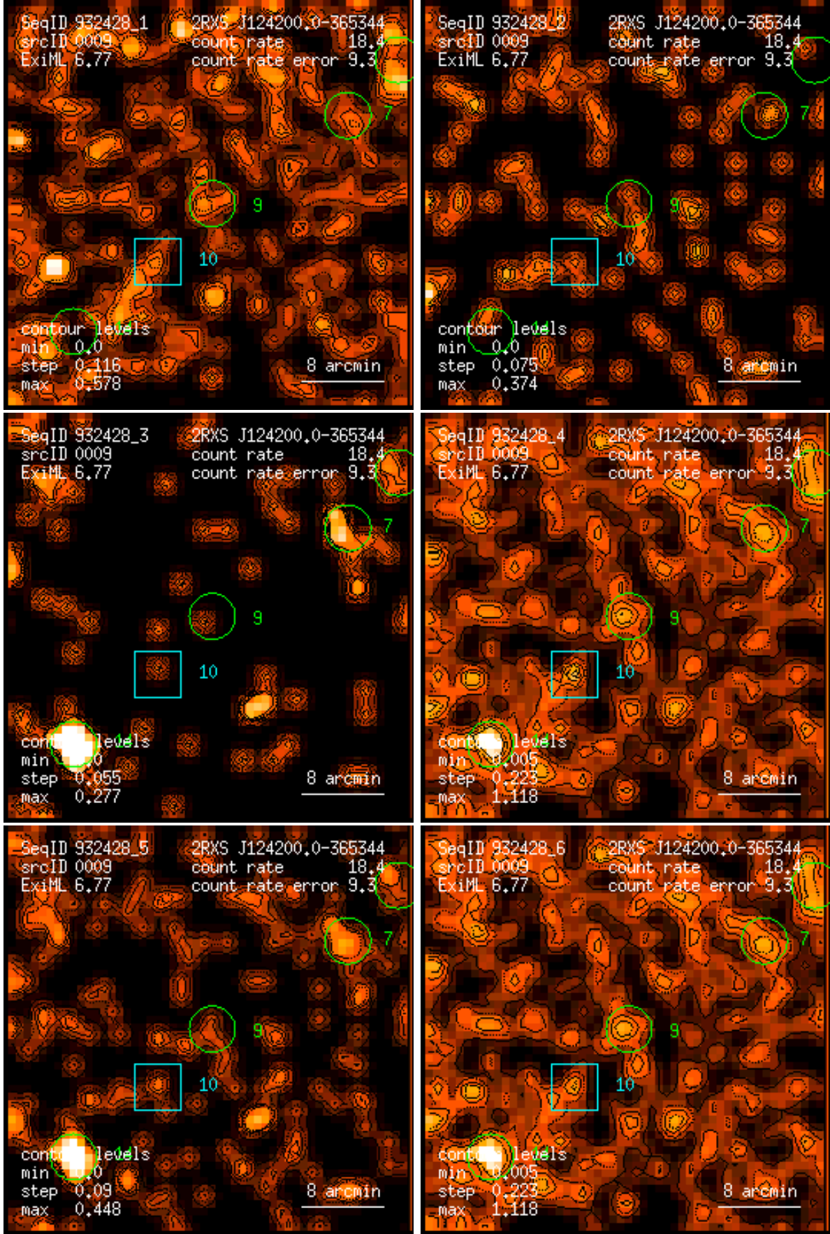
Figure 9: RASS 932428: detection 0009: band rate images, Gaussian filter: (1) PSPC channels 11 – 41, (2) 52 – 90, (3) 91 – 201, (4) 11 – 235, (5) 52 – 201, (6) 11 – 201. Broad band rates in counts/ks. Band rate contour levels in counts/ks/arcmin 2 .
