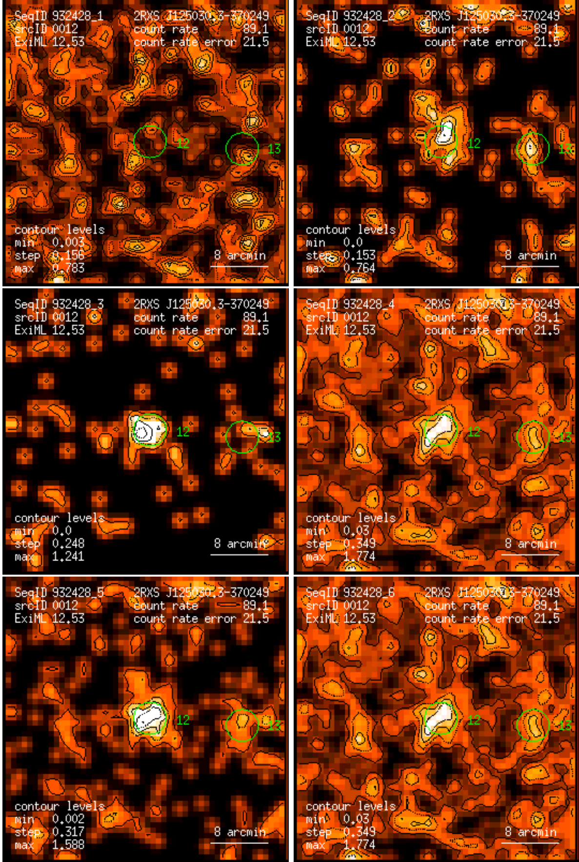
Figure 12: RASS 932428: detection 0012: band rate images, Gaussian filter: (1) PSPC channels 11 – 41, (2) 52 – 90, (3) 91 – 201, (4) 11 – 235, (5) 52 – 201, (6) 11 – 201. Broad band rates in counts/ks. Band rate contour levels in counts/ks/arcmin 2 .
