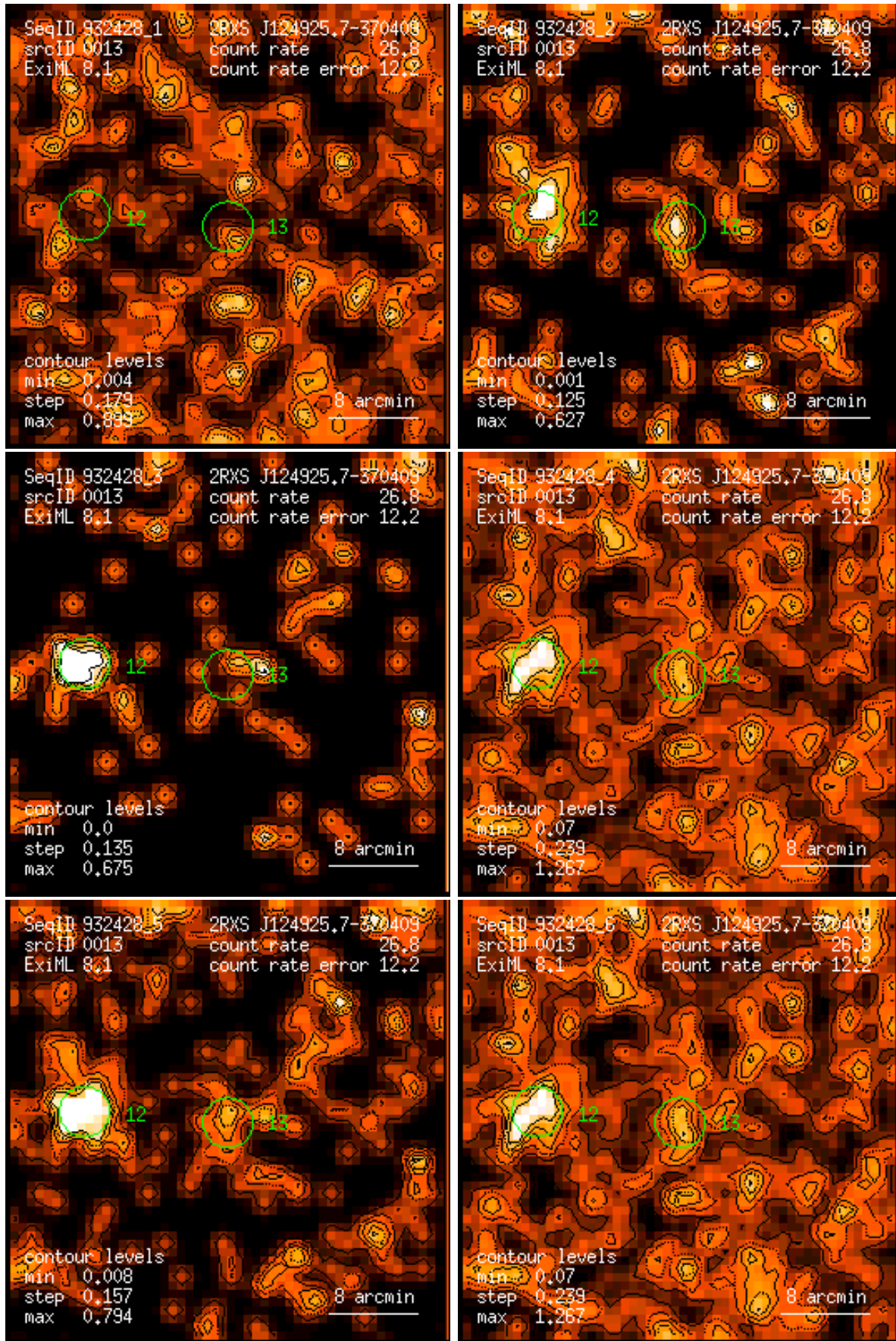
Figure 13: RASS 932428: detection 0013: band rate images, Gaussian filter: (1) PSPC channels 11 – 41, (2) 52 – 90, (3) 91 – 201, (4) 11 – 235, (5) 52 – 201, (6) 11 – 201. Broad band rates in counts/ks. Band rate contour levels in counts/ks/arcmin 2 .
