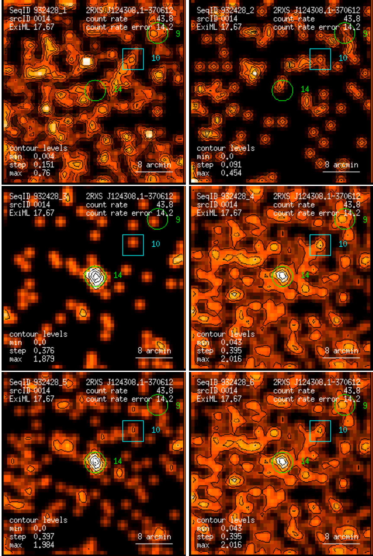
Figure 14: RASS 932428: detection 0014: band rate images, Gaussian filter: (1) PSPC channels 11 – 41, (2) 52 – 90, (3) 91 – 201, (4) 11 – 235, (5) 52 – 201, (6) 11 – 201. Broad band rates in counts/ks. Band rate contour levels in counts/ks/arcmin 2 .
