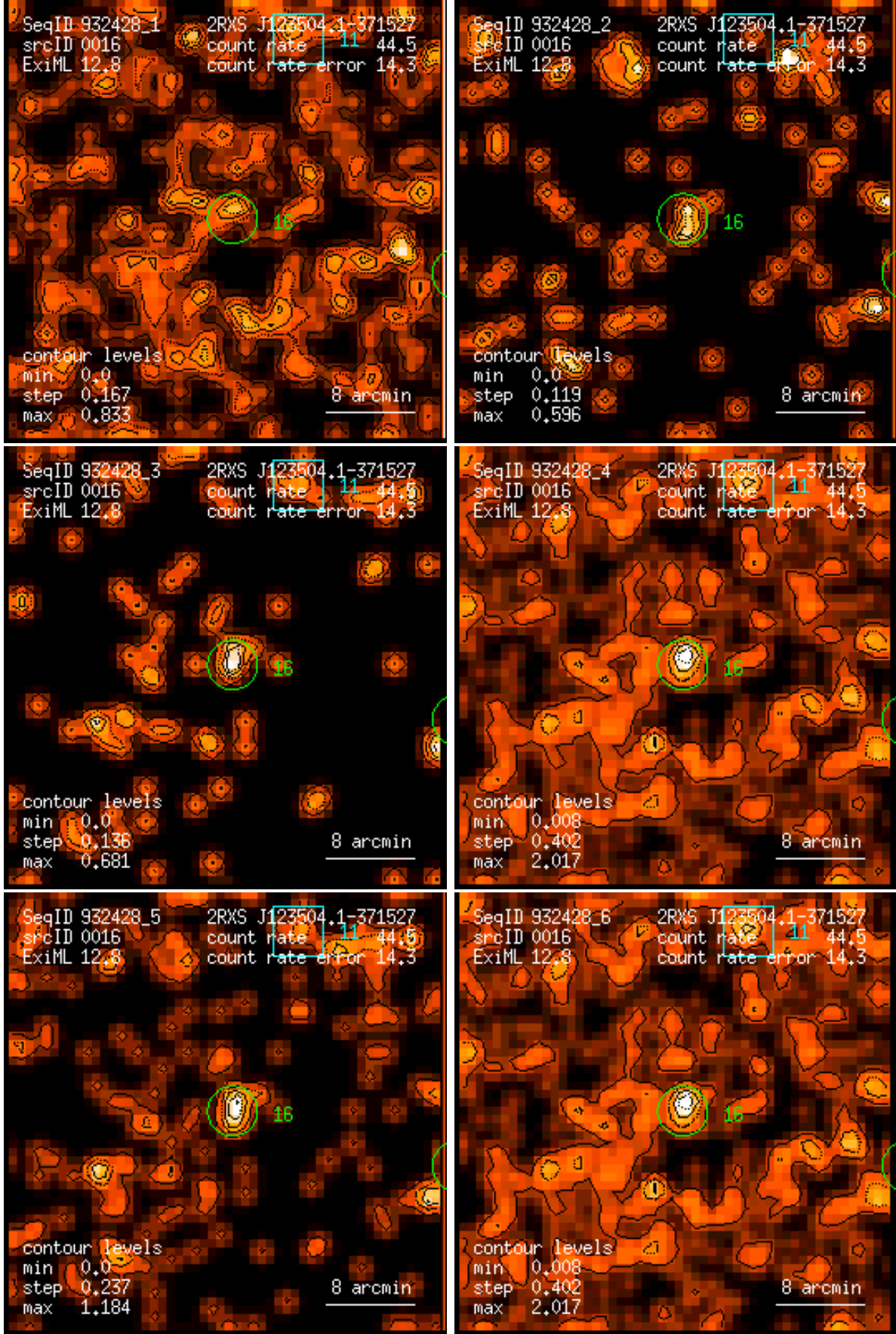
Figure 16: RASS 932428: detection 0016: band rate images, Gaussian filter: (1) PSPC channels 11 – 41, (2) 52 – 90, (3) 91 – 201, (4) 11 – 235, (5) 52 – 201, (6) 11 – 201. Broad band rates in counts/ks. Band rate contour levels in counts/ks/arcmin 2 .
