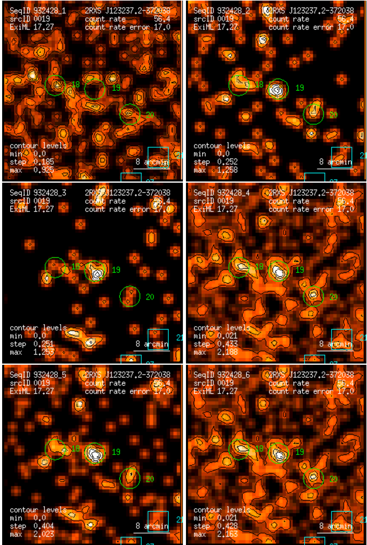
Figure 19: RASS 932428: detection 0019: band rate images, Gaussian filter: (1) PSPC channels 11 – 41, (2) 52 – 90, (3) 91 – 201, (4) 11 – 235, (5) 52 – 201, (6) 11 – 201. Broad band rates in counts/ks. Band rate contour levels in counts/ks/arcmin 2 .
