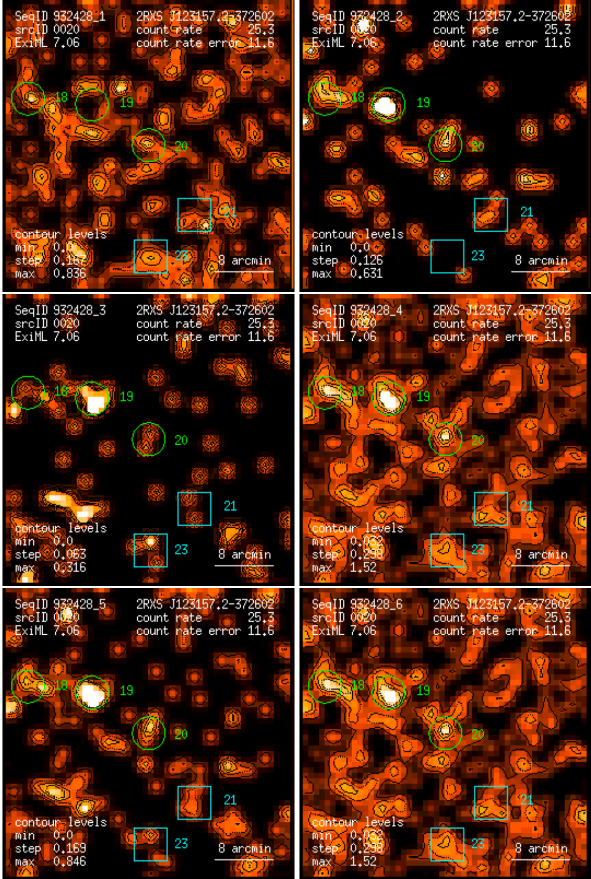
Figure 20: RASS 932428: detection 0020: band rate images, Gaussian filter: (1) PSPC channels 11 – 41, (2) 52 – 90, (3) 91 – 201, (4) 11 – 235, (5) 52 – 201, (6) 11 – 201. Broad band rates in counts/ks. Band rate contour levels in counts/ks/arcmin 2 .
