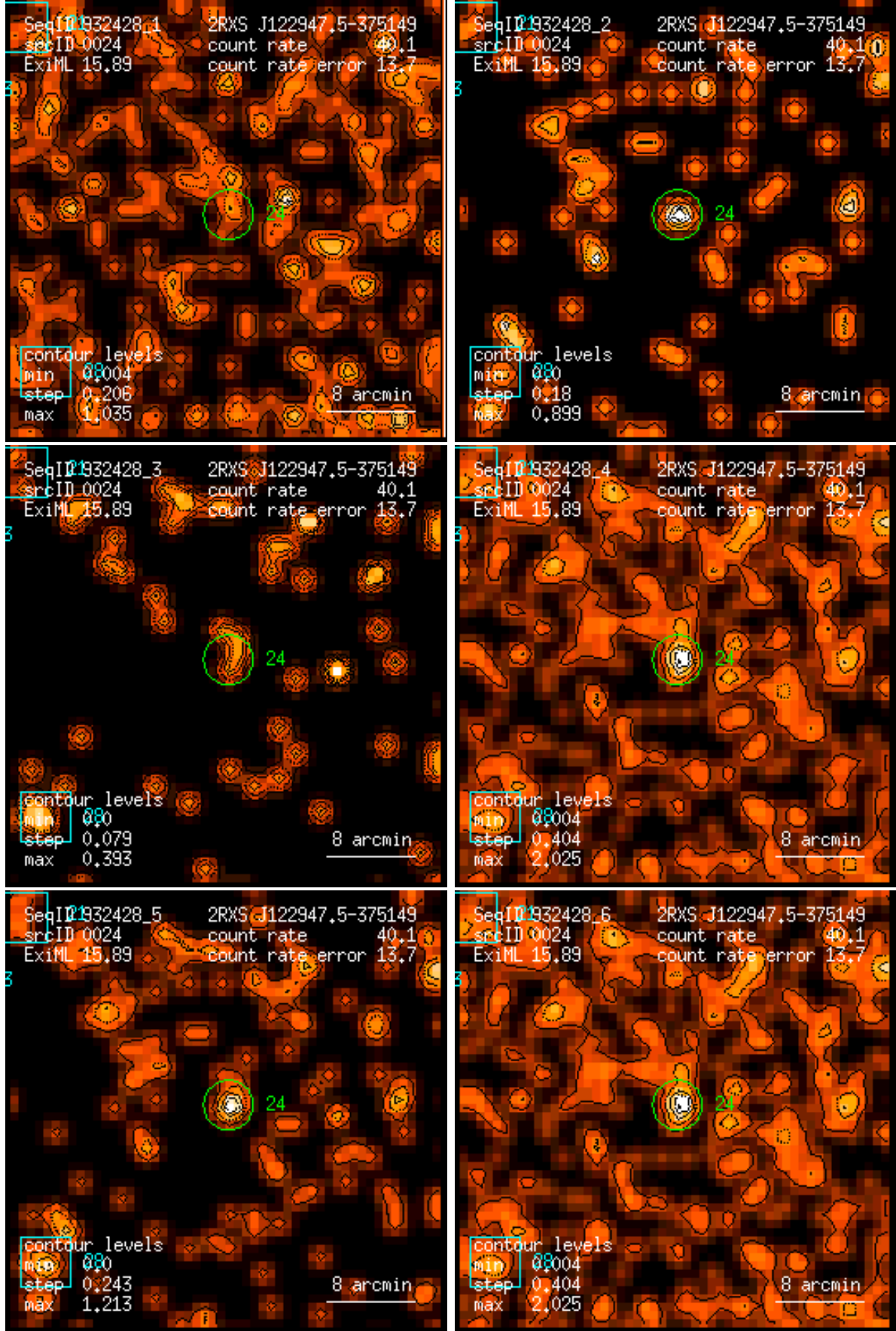
Figure 24: RASS 932428: detection 0024: band rate images, Gaussian filter: (1) PSPC channels 11 – 41, (2) 52 – 90, (3) 91 – 201, (4) 11 – 235, (5) 52 – 201, (6) 11 – 201. Broad band rates in counts/ks. Band rate contour levels in counts/ks/arcmin 2 .
