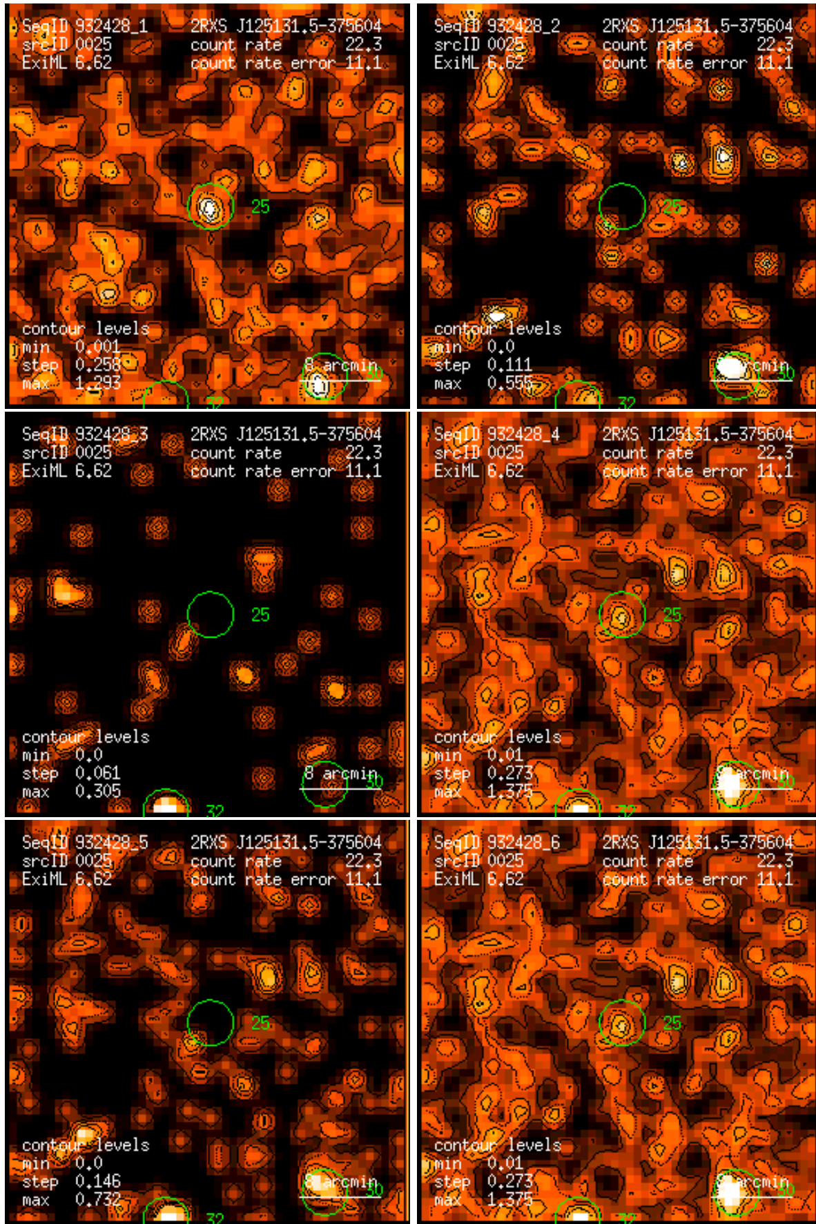
Figure 25: RASS 932428: detection 0025: band rate images, Gaussian filter: (1) PSPC channels 11 – 41, (2) 52 – 90, (3) 91 – 201, (4) 11 – 235, (5) 52 – 201, (6) 11 – 201. Broad band rates in counts/ks. Band rate contour levels in counts/ks/arcmin 2 .
