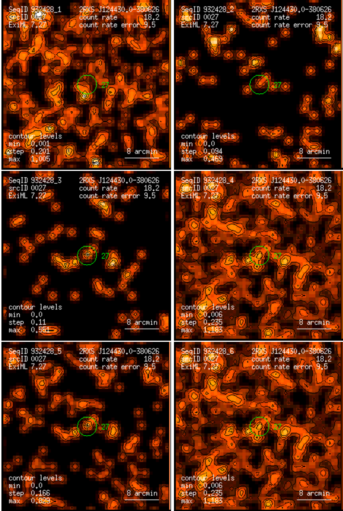
Figure 27: RASS 932428: detection 0027: band rate images, Gaussian filter: (1) PSPC channels 11 – 41, (2) 52 – 90, (3) 91 – 201, (4) 11 – 235, (5) 52 – 201, (6) 11 – 201. Broad band rates in counts/ks. Band rate contour levels in counts/ks/arcmin 2 .
