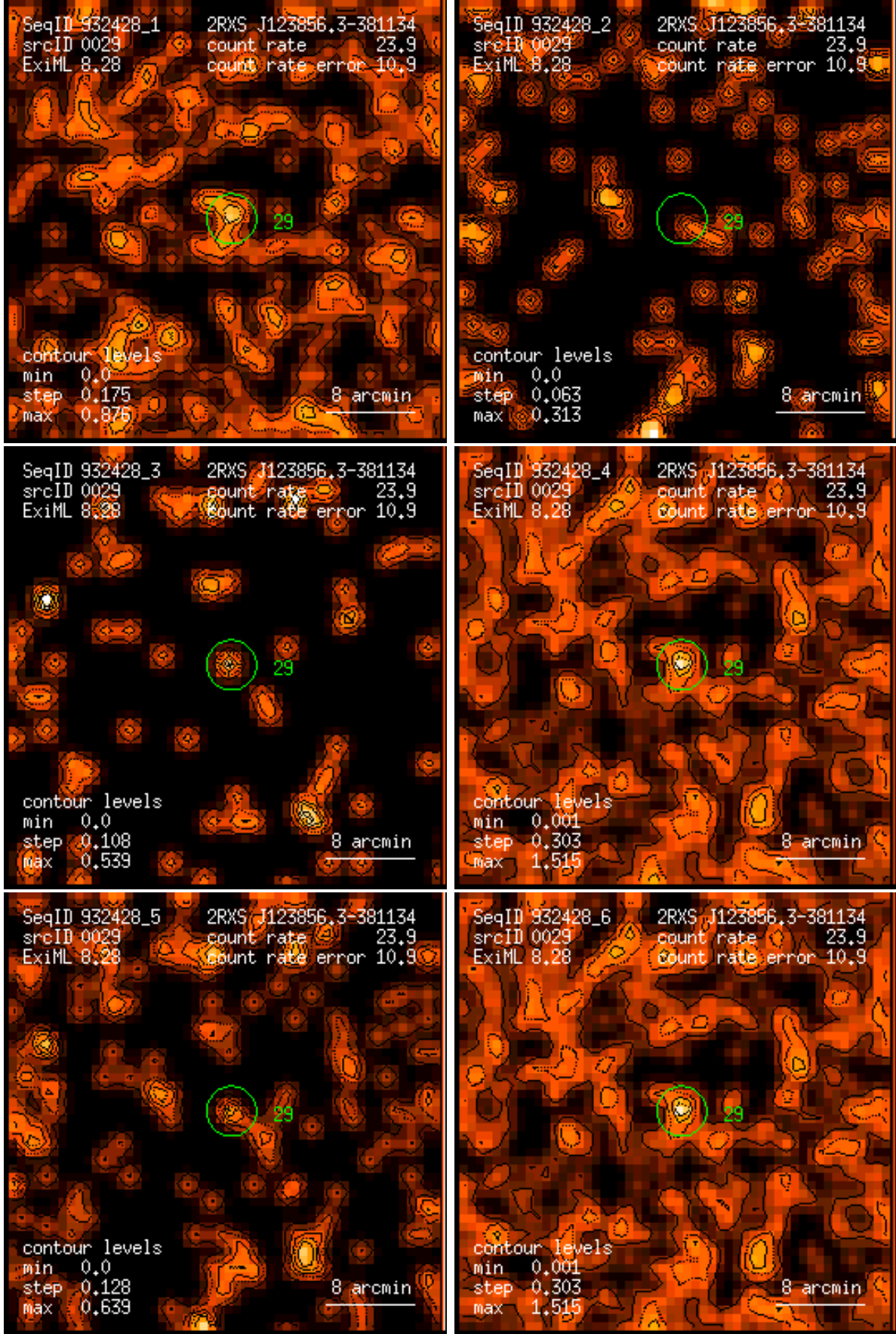
Figure 29: RASS 932428: detection 0029: band rate images, Gaussian filter: (1) PSPC channels 11 – 41, (2) 52 – 90, (3) 91 – 201, (4) 11 – 235, (5) 52 – 201, (6) 11 – 201. Broad band rates in counts/ks. Band rate contour levels in counts/ks/arcmin 2 .
