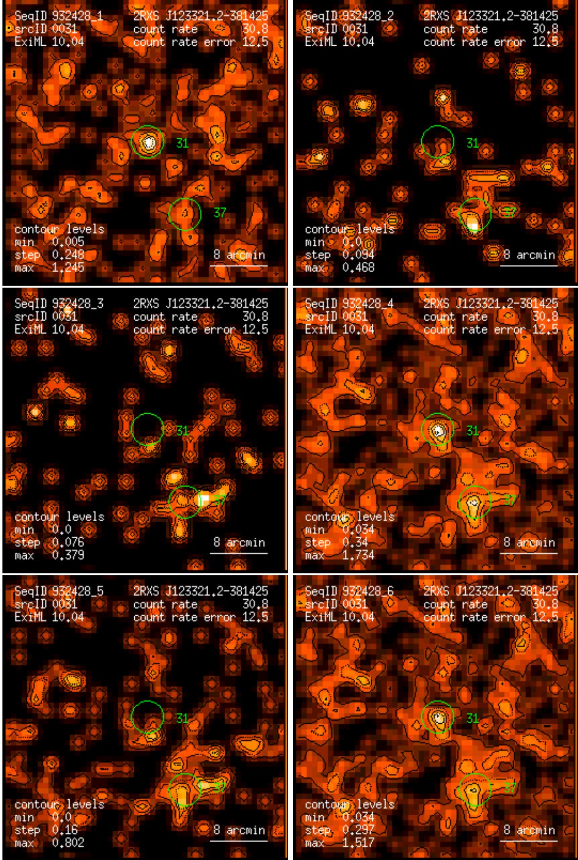
Figure 31: RASS 932428: detection 0031: band rate images, Gaussian filter: (1) PSPC channels 11 – 41, (2) 52 – 90, (3) 91 – 201, (4) 11 – 235, (5) 52 – 201, (6) 11 – 201. Broad band rates in counts/ks. Band rate contour levels in counts/ks/arcmin 2 .
