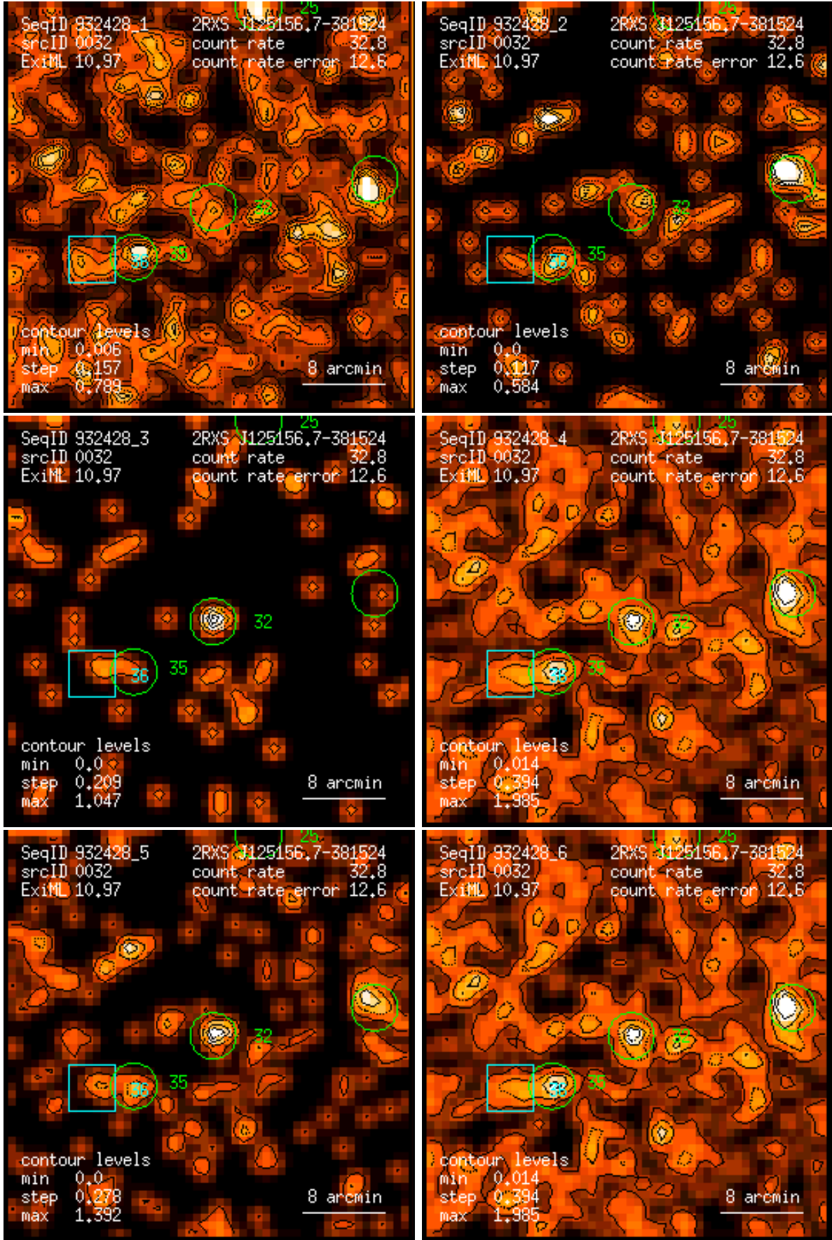
Figure 32: RASS 932428: detection 0032: band rate images, Gaussian filter: (1) PSPC channels 11 – 41, (2) 52 – 90, (3) 91 – 201, (4) 11 – 235, (5) 52 – 201, (6) 11 – 201. Broad band rates in counts/ks. Band rate contour levels in counts/ks/arcmin 2 .
