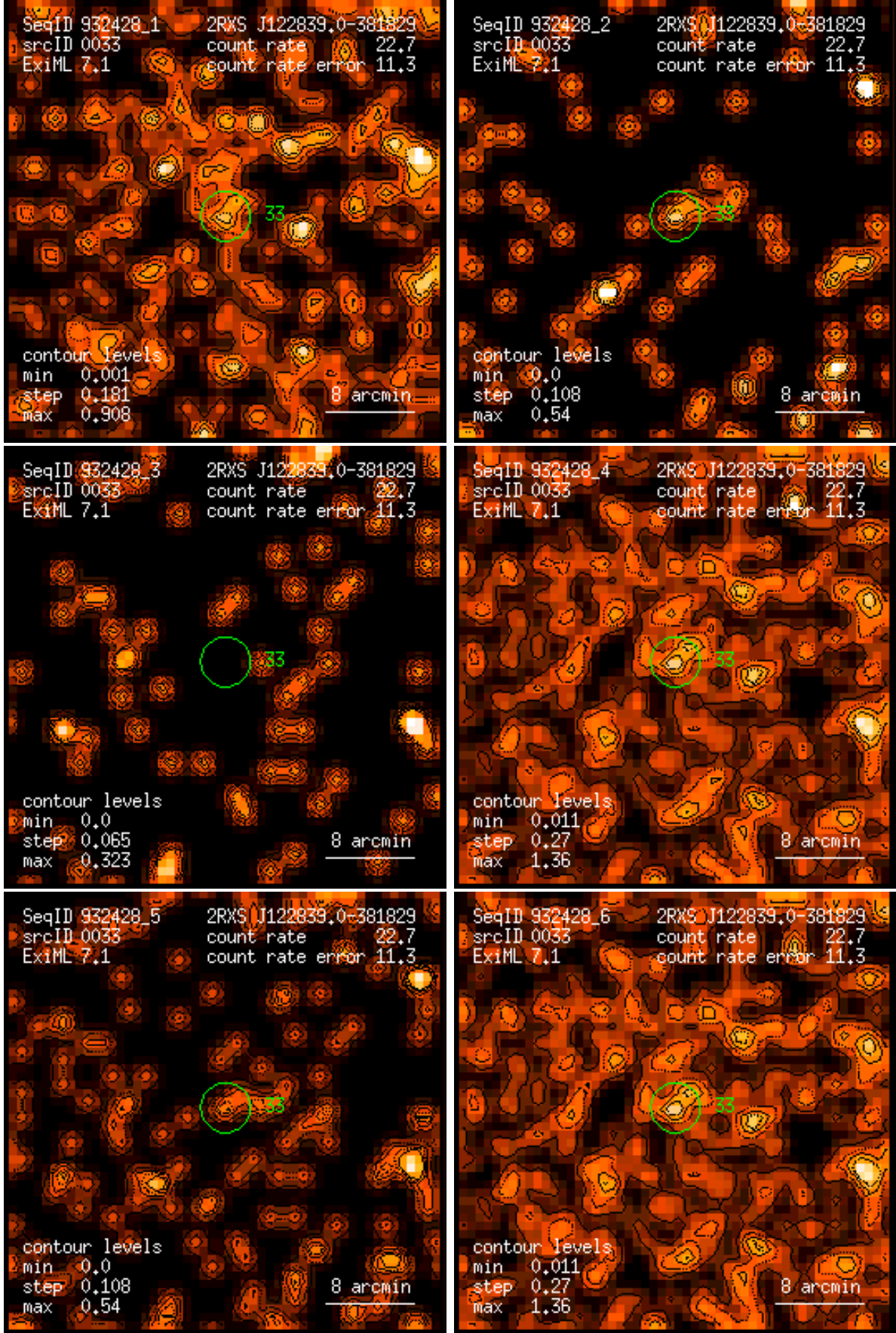
Figure 33: RASS 932428: detection 0033: band rate images, Gaussian filter: (1) PSPC channels 11 – 41, (2) 52 – 90, (3) 91 – 201, (4) 11 – 235, (5) 52 – 201, (6) 11 – 201. Broad band rates in counts/ks. Band rate contour levels in counts/ks/arcmin 2 .
