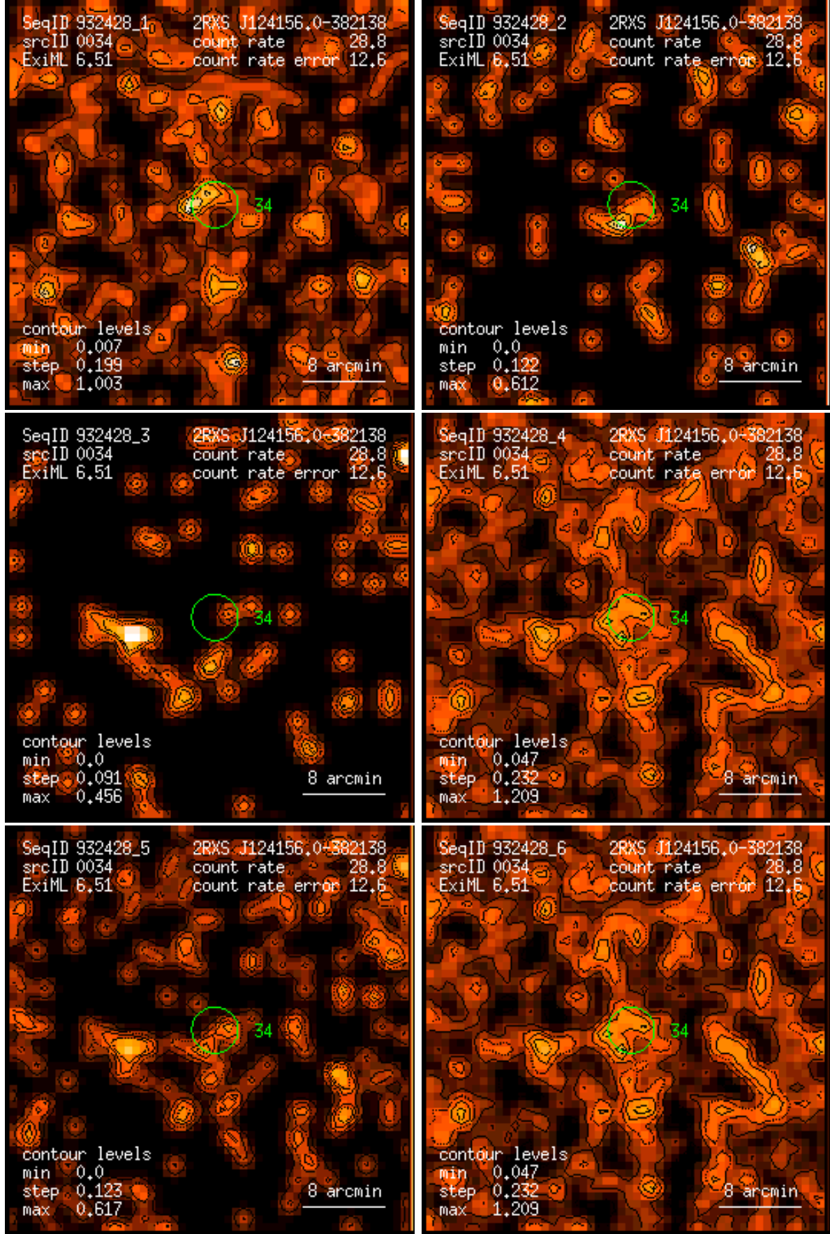
Figure 34: RASS 932428: detection 0034: band rate images, Gaussian filter: (1) PSPC channels 11 – 41, (2) 52 – 90, (3) 91 – 201, (4) 11 – 235, (5) 52 – 201, (6) 11 – 201. Broad band rates in counts/ks. Band rate contour levels in counts/ks/arcmin 2 .
