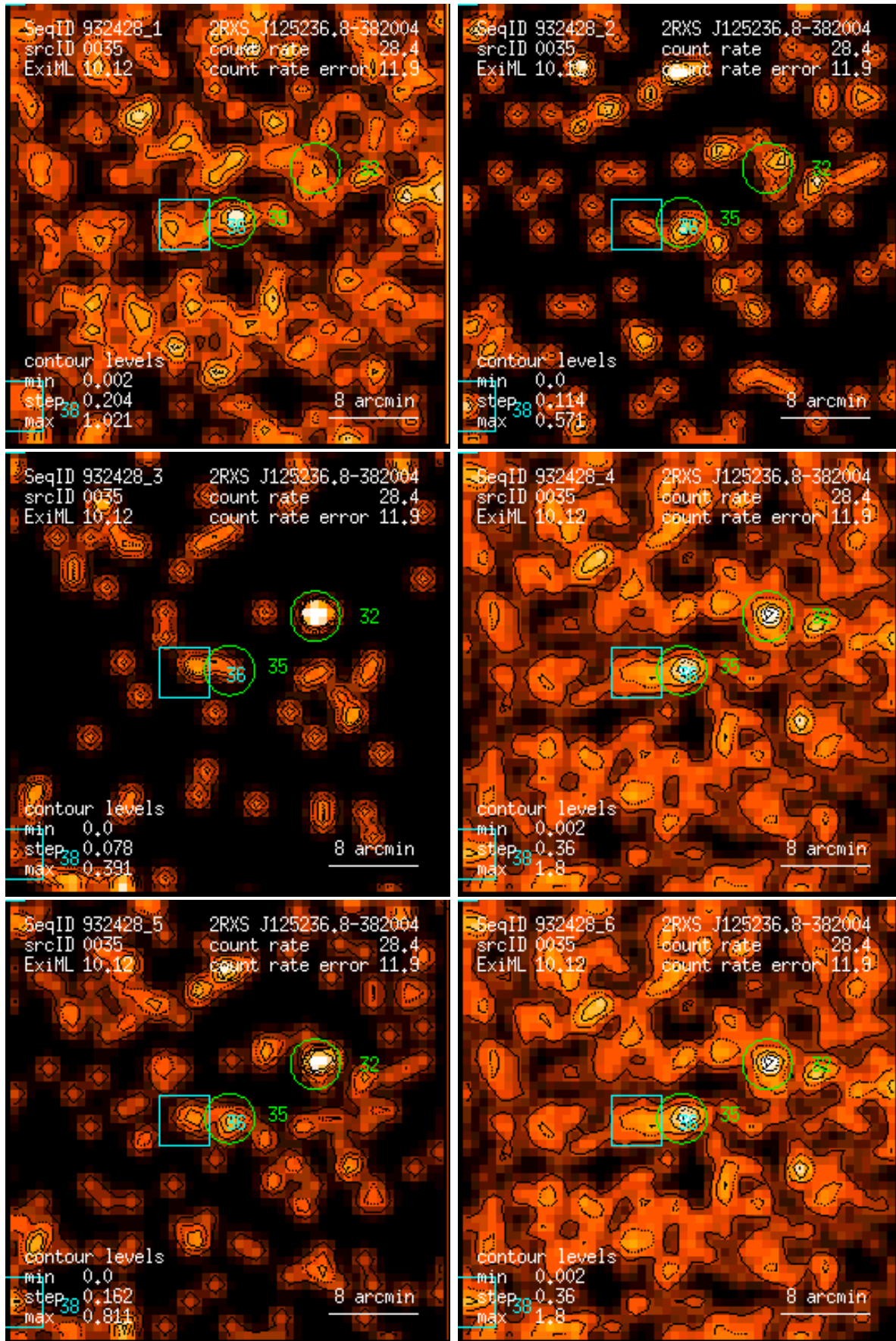
Figure 35: RASS 932428: detection 0035: band rate images, Gaussian filter: (1) PSPC channels 11 – 41, (2) 52 – 90, (3) 91 – 201, (4) 11 – 235, (5) 52 – 201, (6) 11 – 201. Broad band rates in counts/ks. Band rate contour levels in counts/ks/arcmin 2 .
