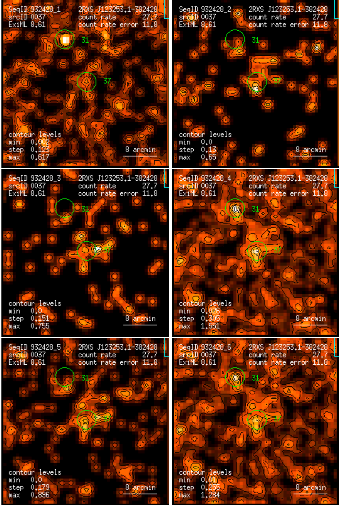
Figure 37: RASS 932428: detection 0037: band rate images, Gaussian filter: (1) PSPC channels 11 – 41, (2) 52 – 90, (3) 91 – 201, (4) 11 – 235, (5) 52 – 201, (6) 11 – 201. Broad band rates in counts/ks. Band rate contour levels in counts/ks/arcmin 2 .
