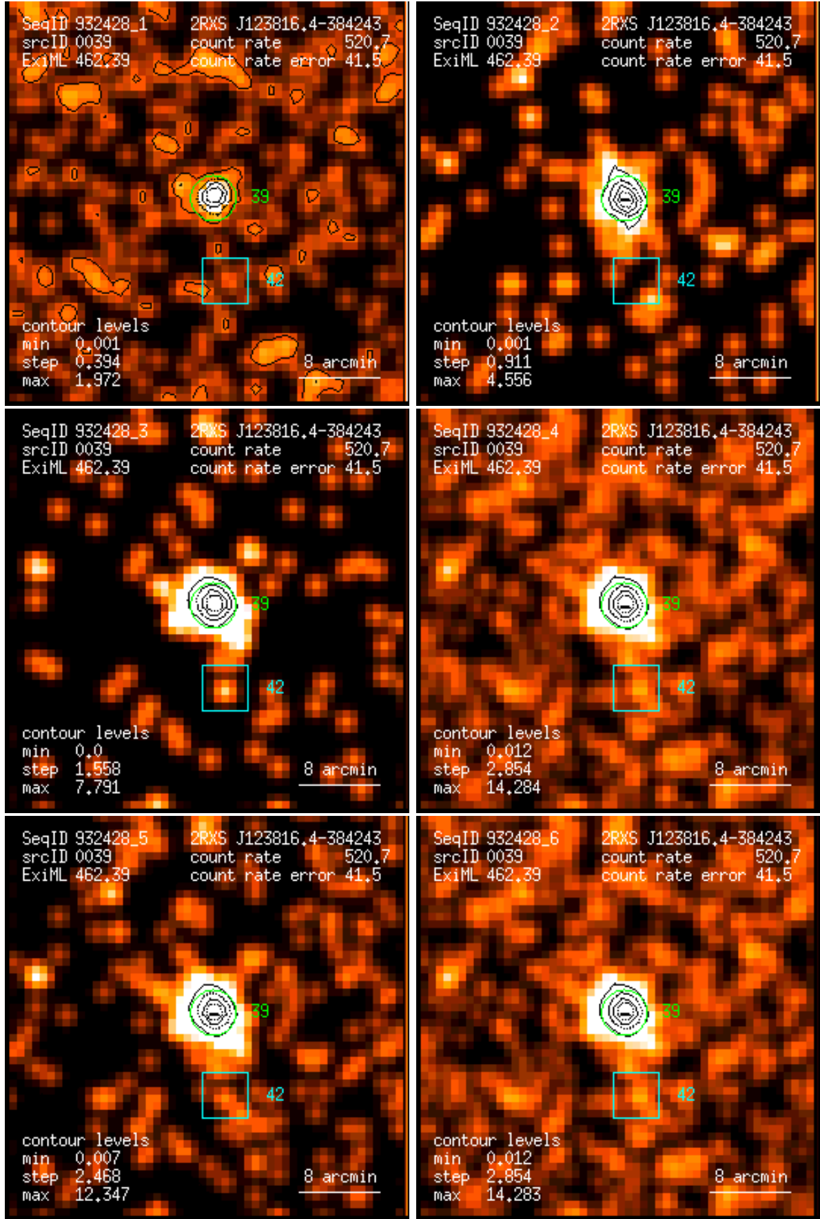
Figure 39: RASS 932428: detection 0039: band rate images, Gaussian filter: (1) PSPC channels 11 – 41, (2) 52 – 90, (3) 91 – 201, (4) 11 – 235, (5) 52 – 201, (6) 11 – 201. Broad band rates in counts/ks. Band rate contour levels in counts/ks/arcmin 2 .
