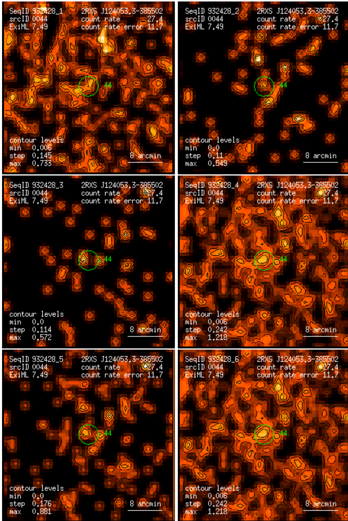
Figure 44: RASS 932428: detection 0044: band rate images, Gaussian filter: (1) PSPC channels 11 – 41, (2) 52 – 90, (3) 91 – 201, (4) 11 – 235, (5) 52 – 201, (6) 11 – 201. Broad band rates in counts/ks. Band rate contour levels in counts/ks/arcmin 2 .
