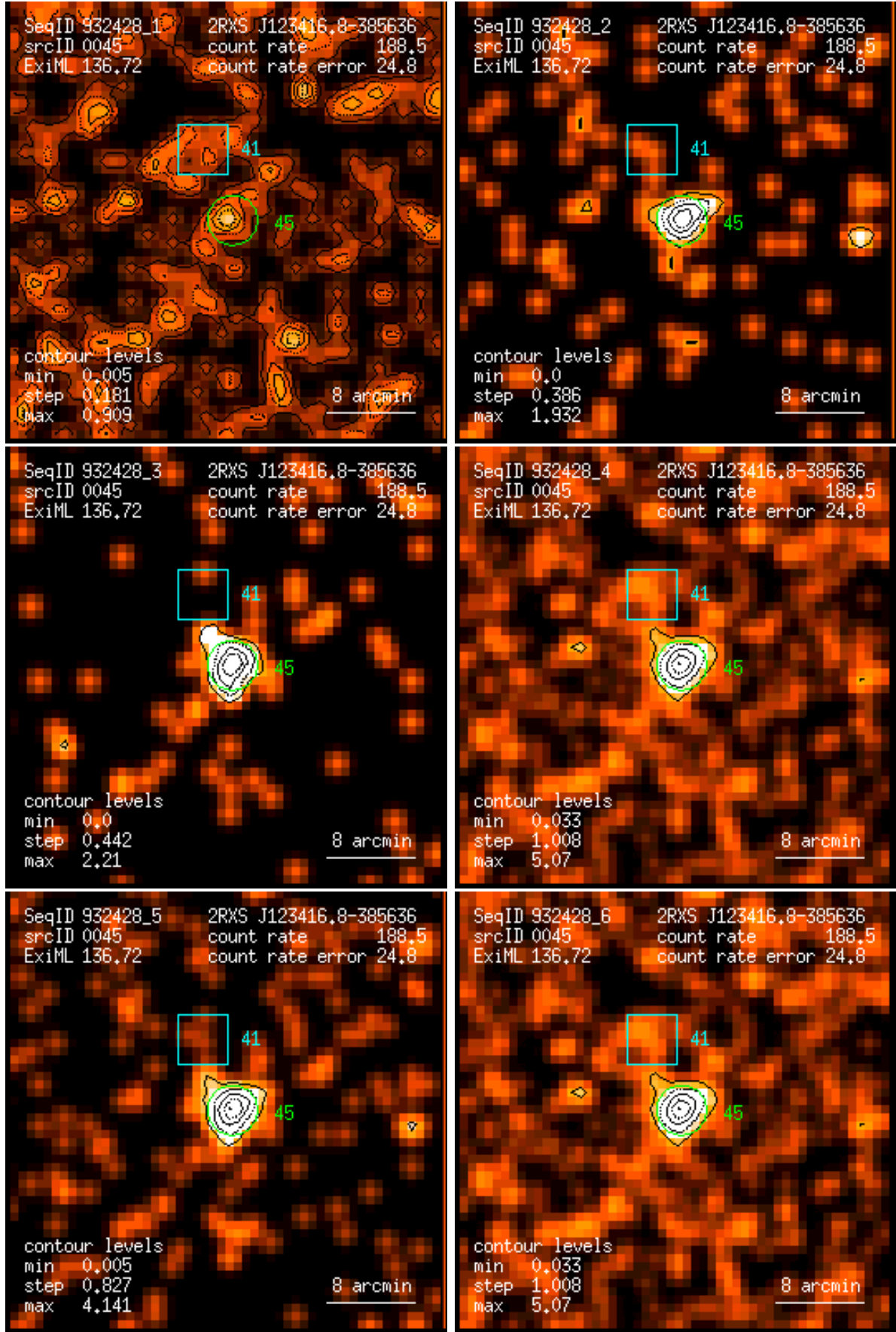
Figure 45: RASS 932428: detection 0045: band rate images, Gaussian filter: (1) PSPC channels 11 – 41, (2) 52 – 90, (3) 91 – 201, (4) 11 – 235, (5) 52 – 201, (6) 11 – 201. Broad band rates in counts/ks. Band rate contour levels in counts/ks/arcmin 2 .
