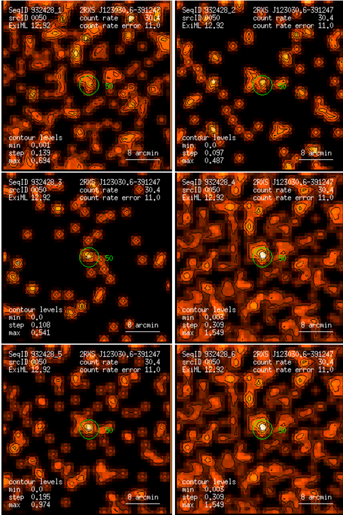
Figure 50: RASS 932428: detection 0050: band rate images, Gaussian filter: (1) PSPC channels 11 – 41, (2) 52 – 90, (3) 91 – 201, (4) 11 – 235, (5) 52 – 201, (6) 11 – 201. Broad band rates in counts/ks. Band rate contour levels in counts/ks/arcmin 2 .
