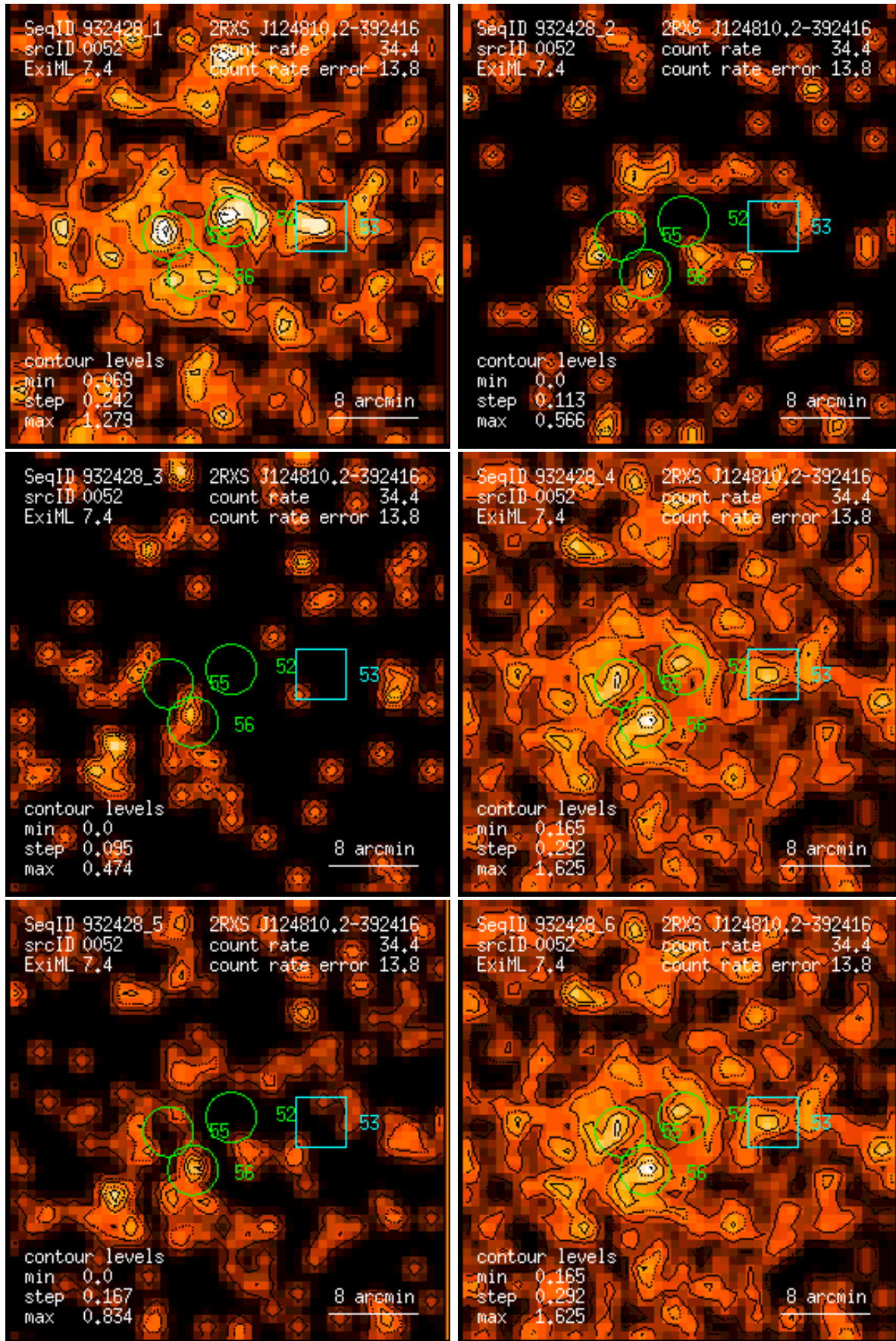
Figure 52: RASS 932428: detection 0052: band rate images, Gaussian filter: (1) PSPC channels 11 – 41, (2) 52 – 90, (3) 91 – 201, (4) 11 – 235, (5) 52 – 201, (6) 11 – 201. Broad band rates in counts/ks. Band rate contour levels in counts/ks/arcmin 2 .
