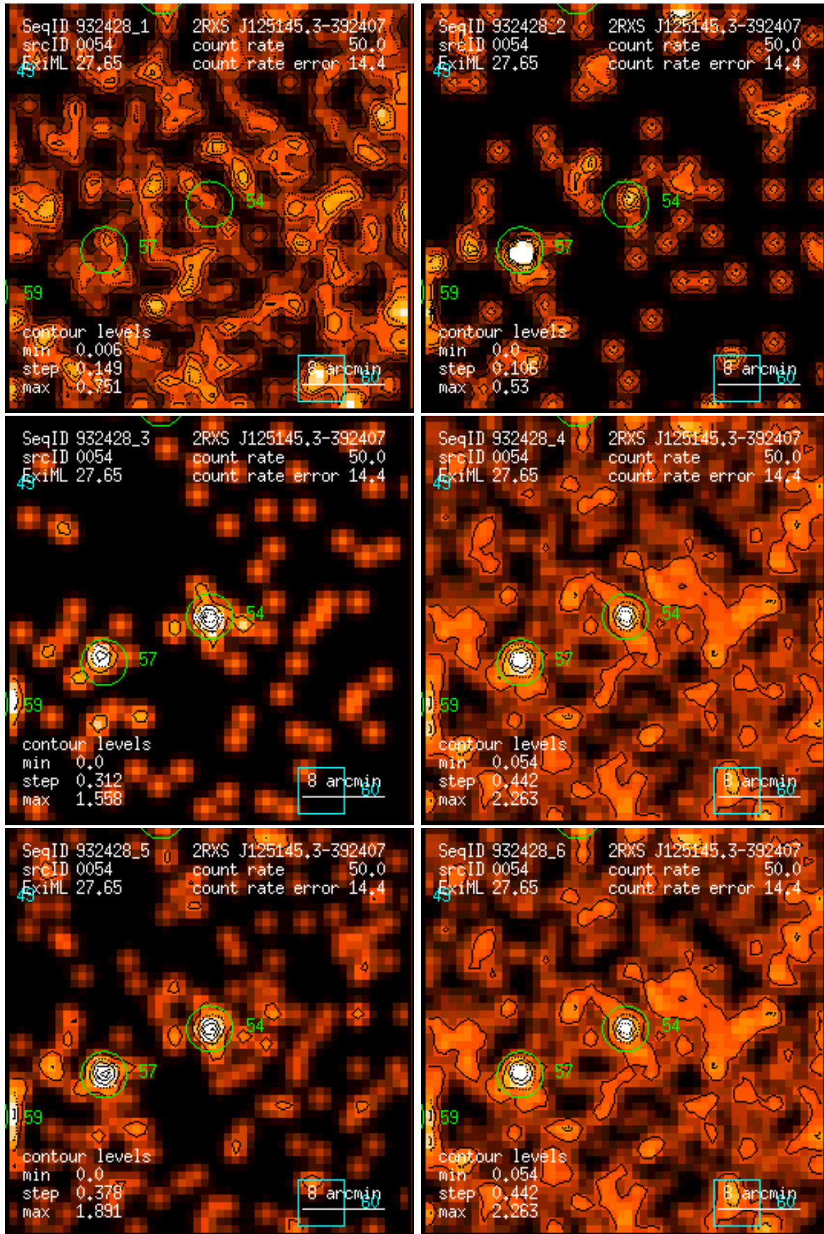
Figure 54: RASS 932428: detection 0054: band rate images, Gaussian filter: (1) PSPC channels 11 – 41, (2) 52 – 90, (3) 91 – 201, (4) 11 – 235, (5) 52 – 201, (6) 11 – 201. Broad band rates in counts/ks. Band rate contour levels in counts/ks/arcmin 2 .
