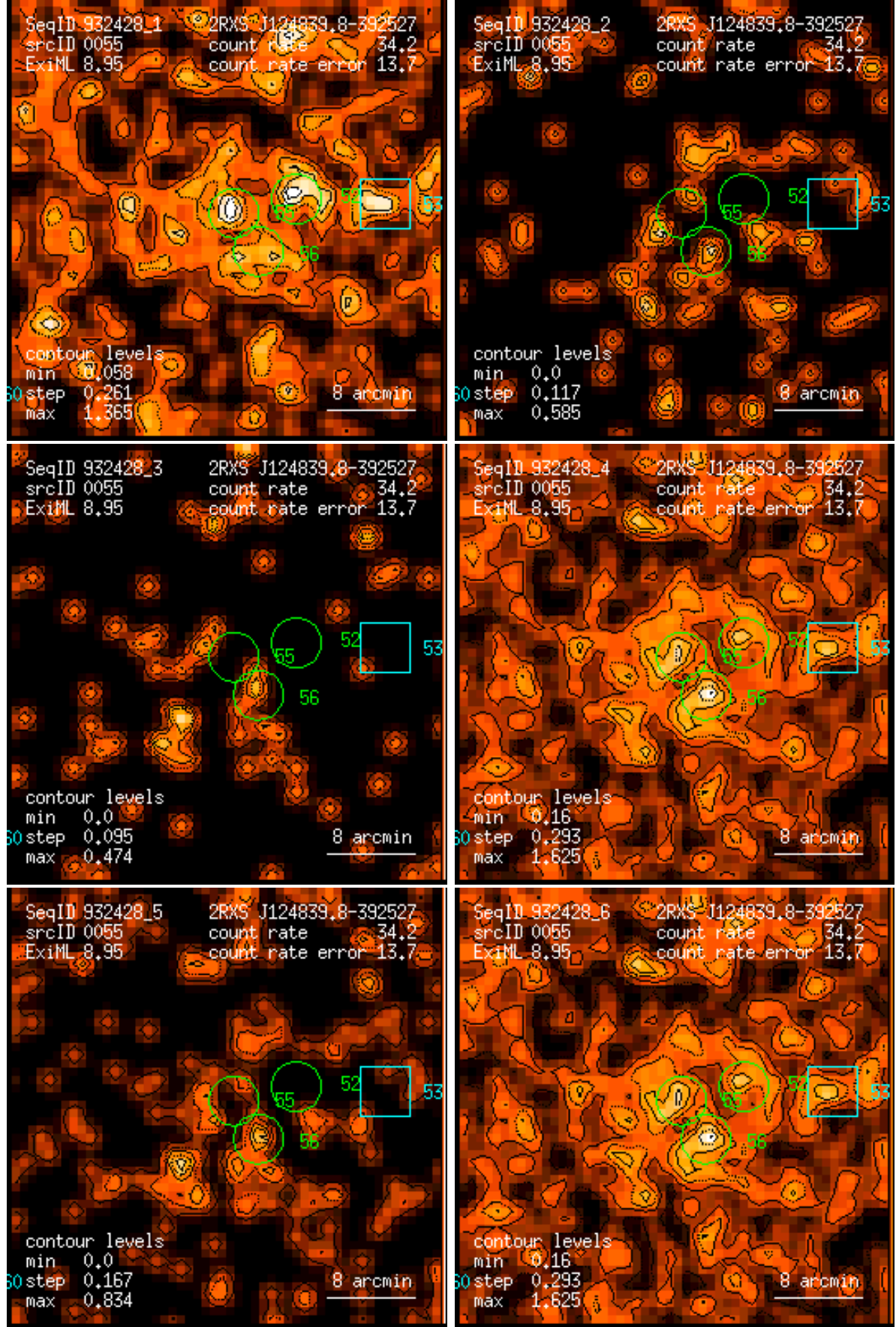
Figure 55: RASS 932428: detection 0055: band rate images, Gaussian filter: (1) PSPC channels 11 – 41, (2) 52 – 90, (3) 91 – 201, (4) 11 – 235, (5) 52 – 201, (6) 11 – 201. Broad band rates in counts/ks. Band rate contour levels in counts/ks/arcmin 2 .
