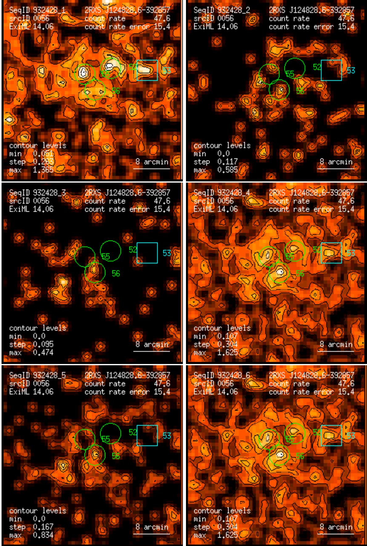
Figure 56: RASS 932428: detection 0056: band rate images, Gaussian filter: (1) PSPC channels 11 – 41, (2) 52 – 90, (3) 91 – 201, (4) 11 – 235, (5) 52 – 201, (6) 11 – 201. Broad band rates in counts/ks. Band rate contour levels in counts/ks/arcmin 2 .
