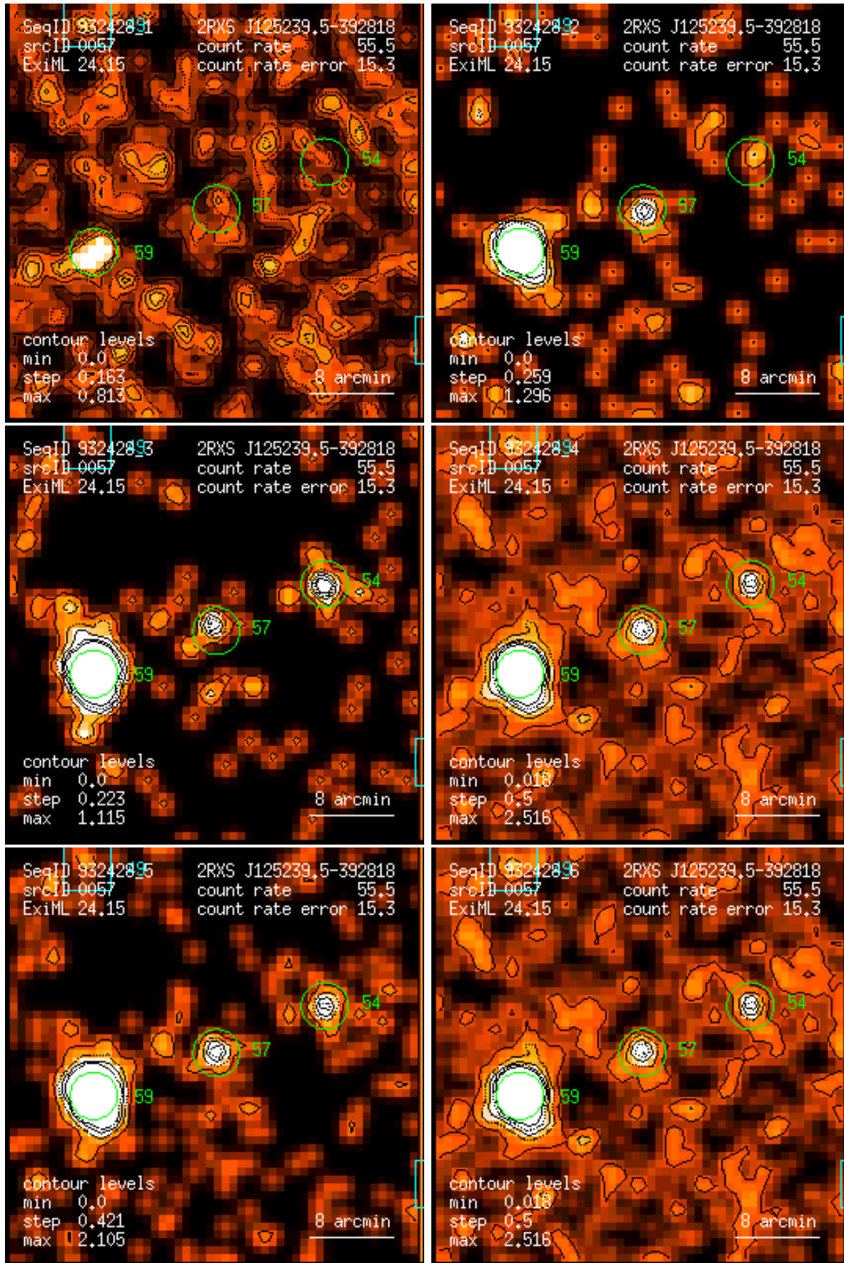
Figure 57: RASS 932428: detection 0057: band rate images, Gaussian filter: (1) PSPC channels 11 – 41, (2) 52 – 90, (3) 91 – 201, (4) 11 – 235, (5) 52 – 201, (6) 11 – 201. Broad band rates in counts/ks. Band rate contour levels in counts/ks/arcmin 2 .
