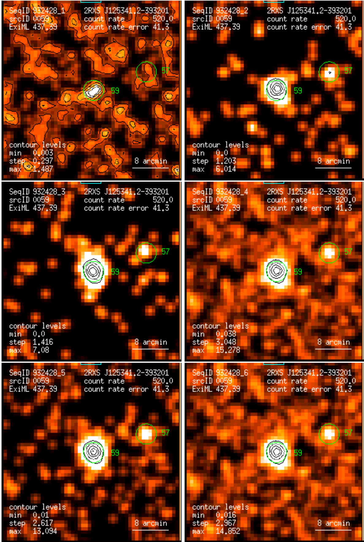
Figure 59: RASS 932428: detection 0059: band rate images, Gaussian filter: (1) PSPC channels 11 – 41, (2) 52 – 90, (3) 91 – 201, (4) 11 – 235, (5) 52 – 201, (6) 11 – 201. Broad band rates in counts/ks. Band rate contour levels in counts/ks/arcmin 2 .
