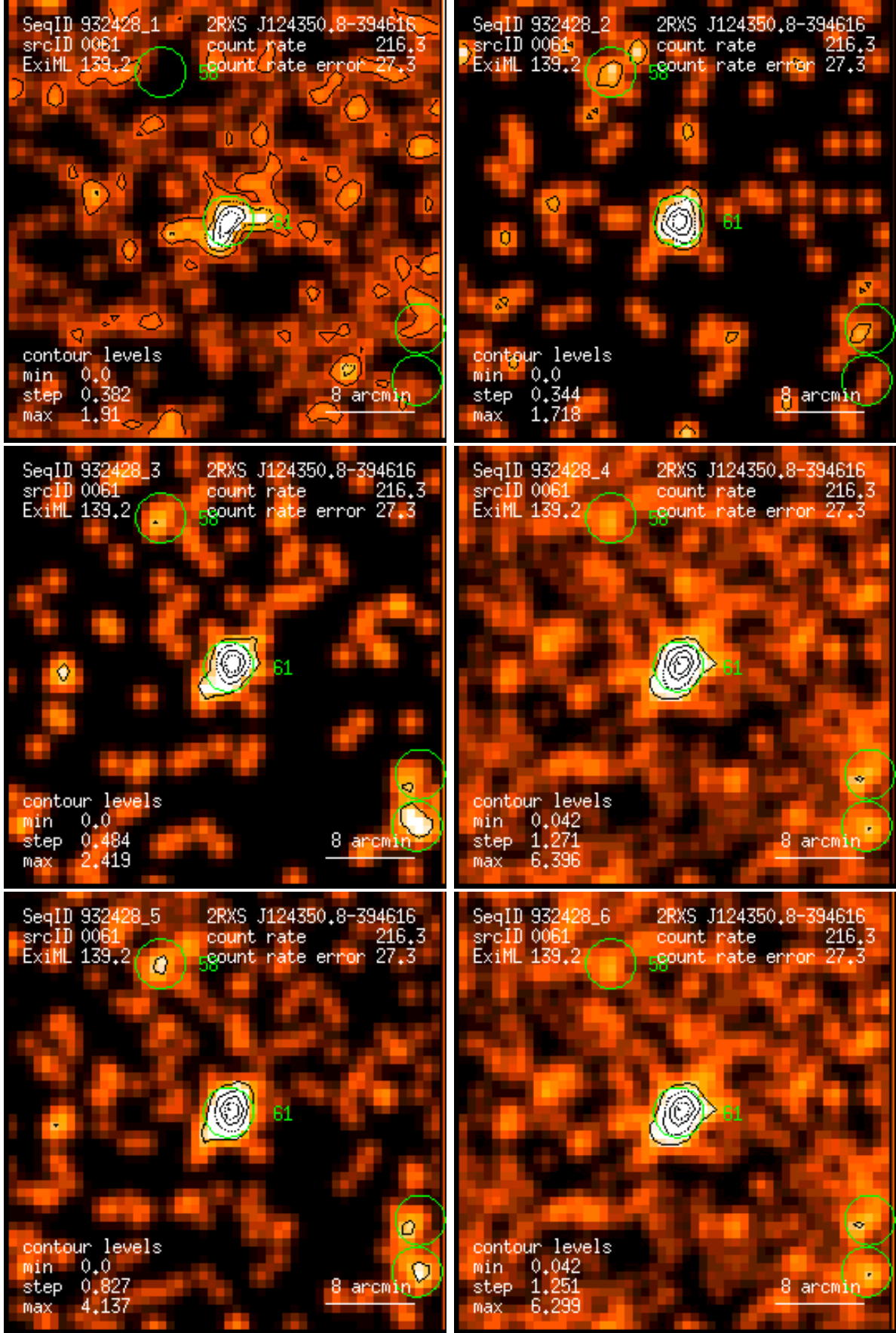
Figure 61: RASS 932428: detection 0061: band rate images, Gaussian filter: (1) PSPC channels 11 – 41, (2) 52 – 90, (3) 91 – 201, (4) 11 – 235, (5) 52 – 201, (6) 11 – 201. Broad band rates in counts/ks. Band rate contour levels in counts/ks/arcmin 2 .
