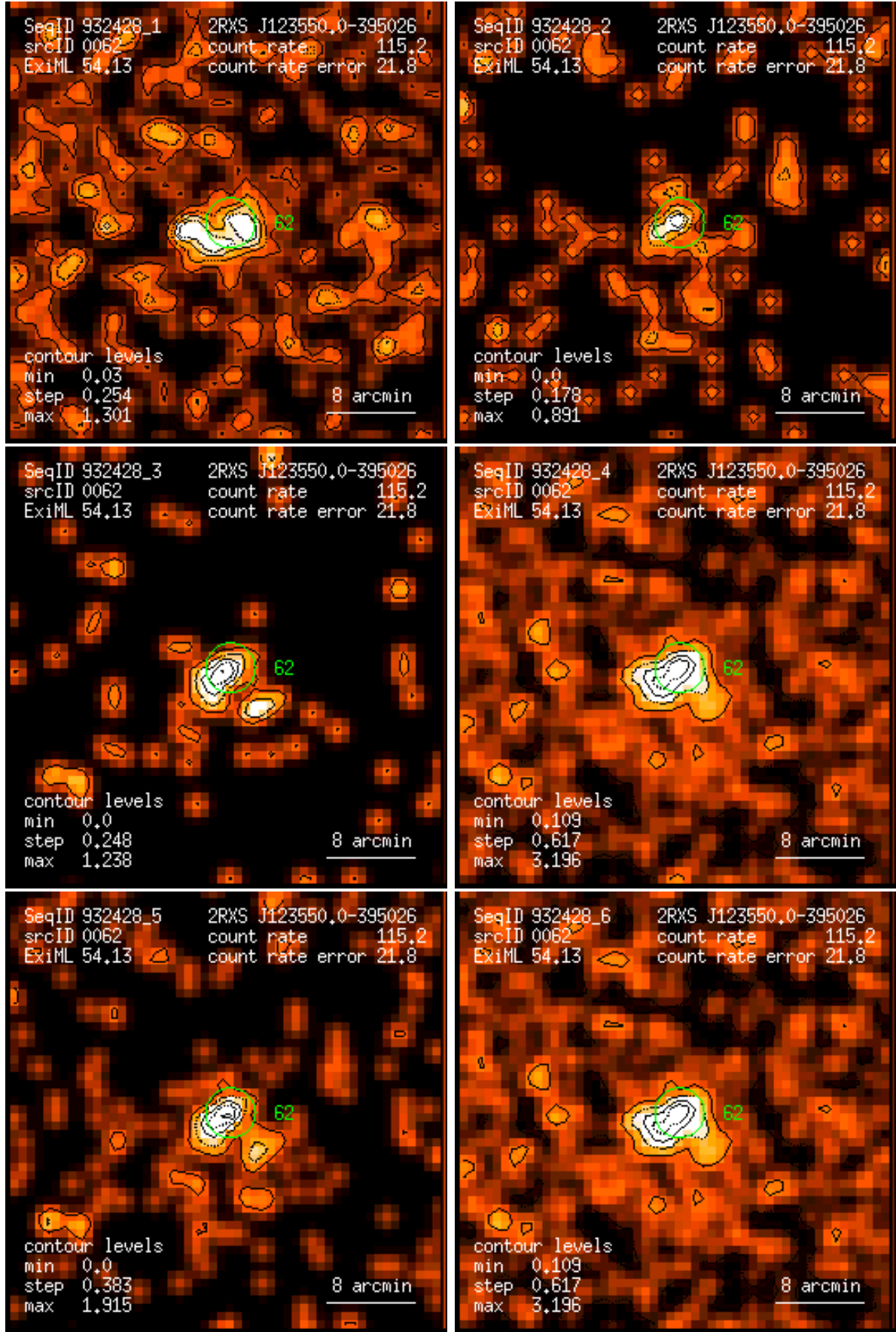
Figure 62: RASS 932428: detection 0062: band rate images, Gaussian filter: (1) PSPC channels 11 – 41, (2) 52 – 90, (3) 91 – 201, (4) 11 – 235, (5) 52 – 201, (6) 11 – 201. Broad band rates in counts/ks. Band rate contour levels in counts/ks/arcmin 2 .
