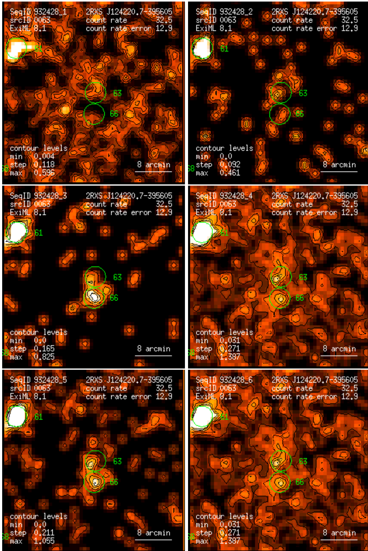
Figure 63: RASS 932428: detection 0063: band rate images, Gaussian filter: (1) PSPC channels 11 – 41, (2) 52 – 90, (3) 91 – 201, (4) 11 – 235, (5) 52 – 201, (6) 11 – 201. Broad band rates in counts/ks. Band rate contour levels in counts/ks/arcmin 2 .
