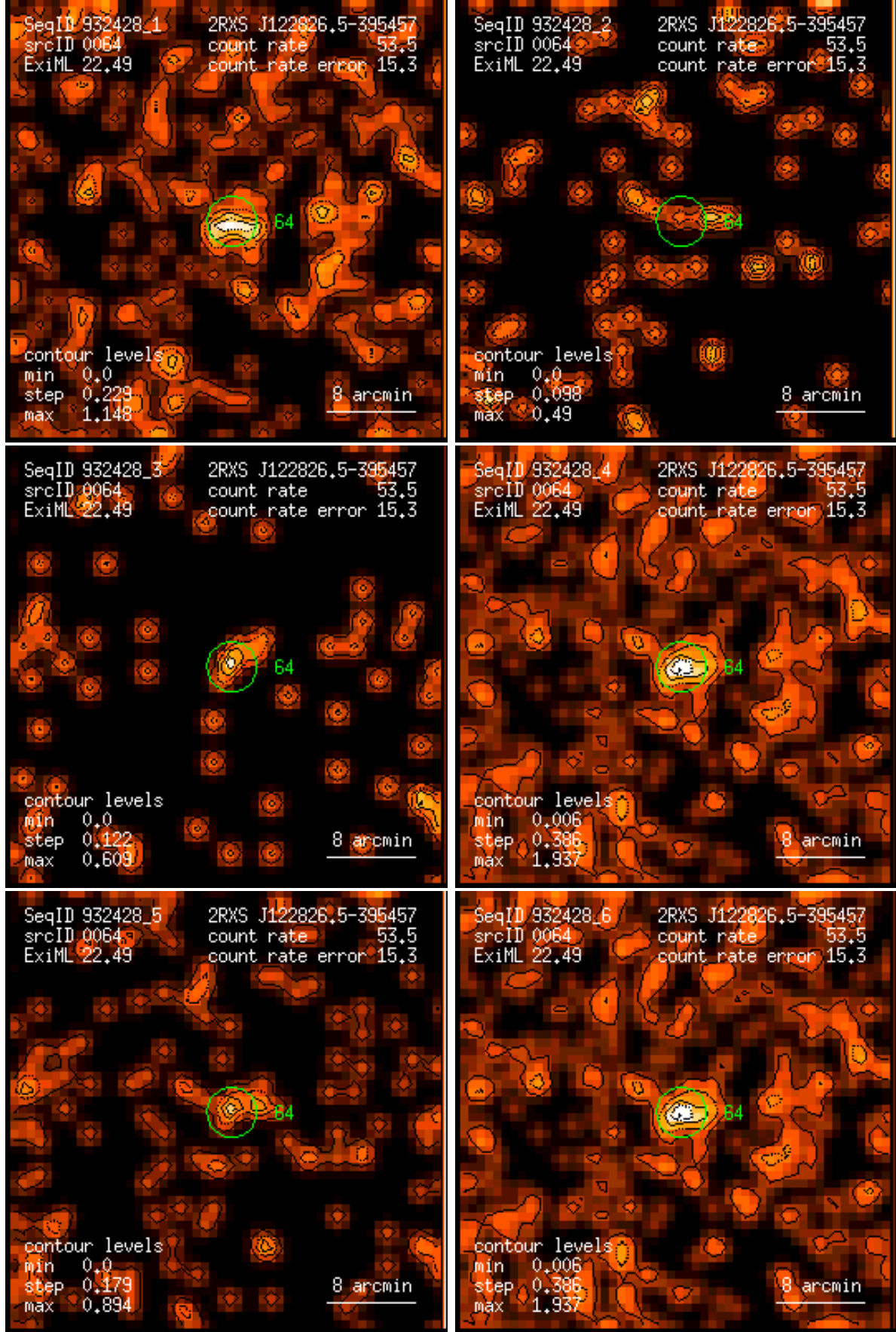
Figure 64: RASS 932428: detection 0064: band rate images, Gaussian filter: (1) PSPC channels 11 – 41, (2) 52 – 90, (3) 91 – 201, (4) 11 – 235, (5) 52 – 201, (6) 11 – 201. Broad band rates in counts/ks. Band rate contour levels in counts/ks/arcmin 2 .
