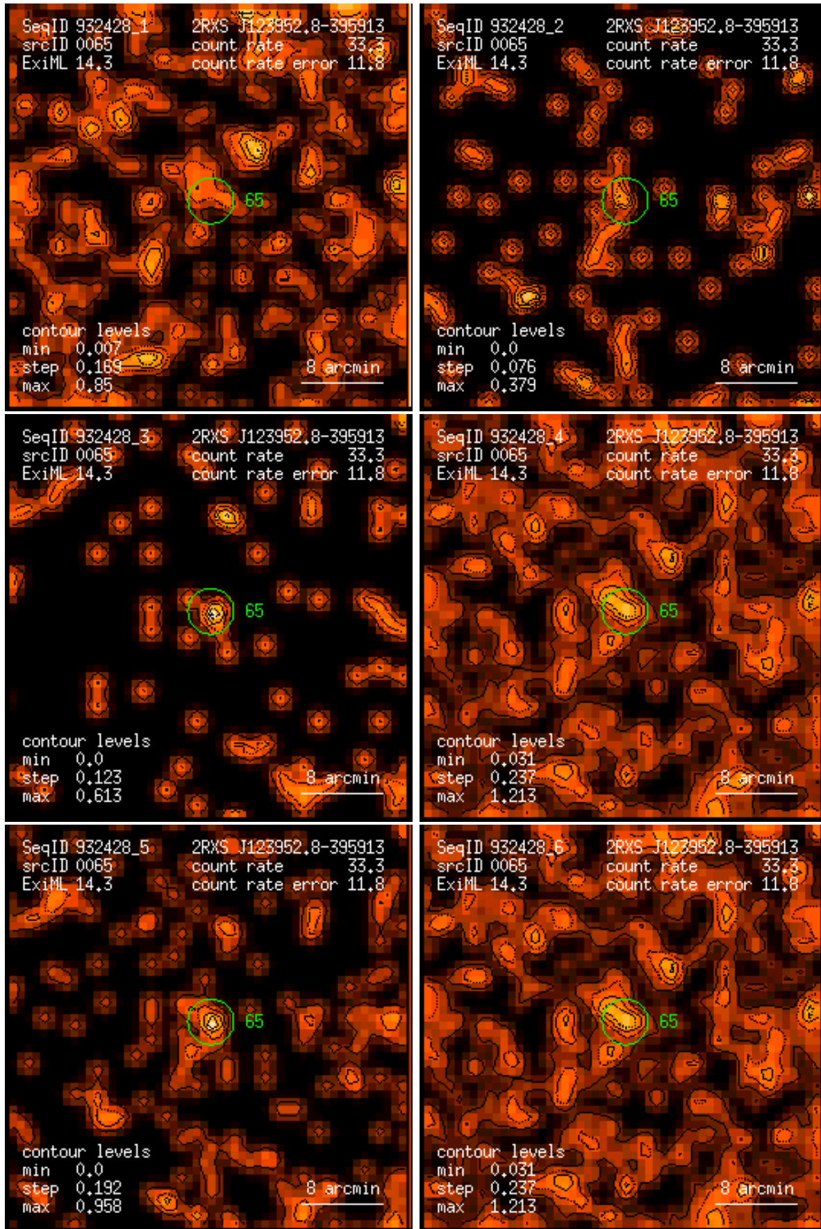
Figure 65: RASS 932428: detection 0065: band rate images, Gaussian filter: (1) PSPC channels 11 – 41, (2) 52 – 90, (3) 91 – 201, (4) 11 – 235, (5) 52 – 201, (6) 11 – 201. Broad band rates in counts/ks. Band rate contour levels in counts/ks/arcmin 2 .
