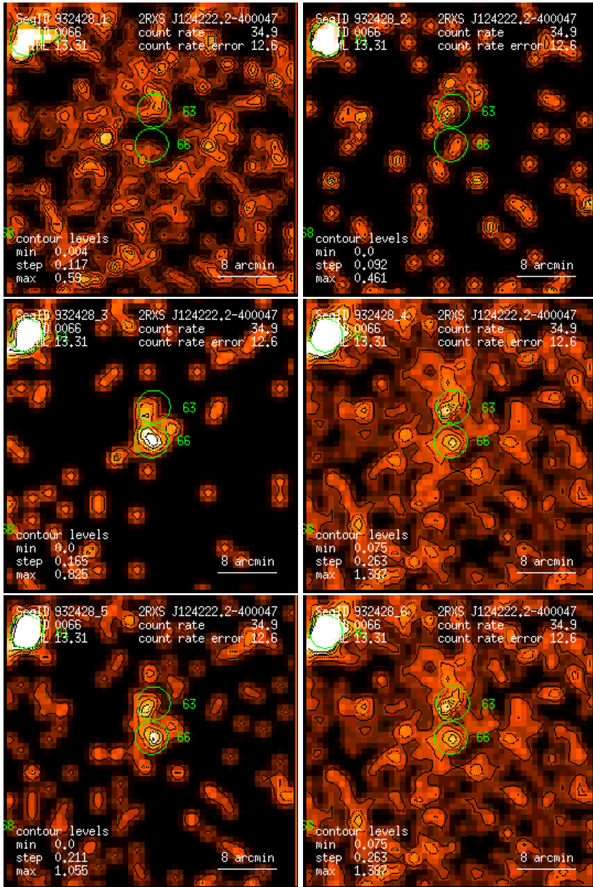
Figure 66: RASS 932428: detection 0066: band rate images, Gaussian filter: (1) PSPC channels 11 – 41, (2) 52 – 90, (3) 91 – 201, (4) 11 – 235, (5) 52 – 201, (6) 11 – 201. Broad band rates in counts/ks. Band rate contour levels in counts/ks/arcmin 2 .
