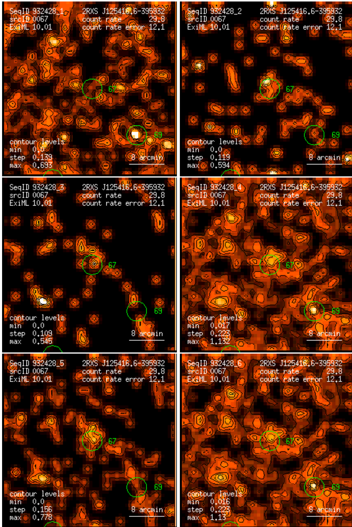
Figure 67: RASS 932428: detection 0067: band rate images, Gaussian filter: (1) PSPC channels 11 – 41, (2) 52 – 90, (3) 91 – 201, (4) 11 – 235, (5) 52 – 201, (6) 11 – 201. Broad band rates in counts/ks. Band rate contour levels in counts/ks/arcmin 2 .
