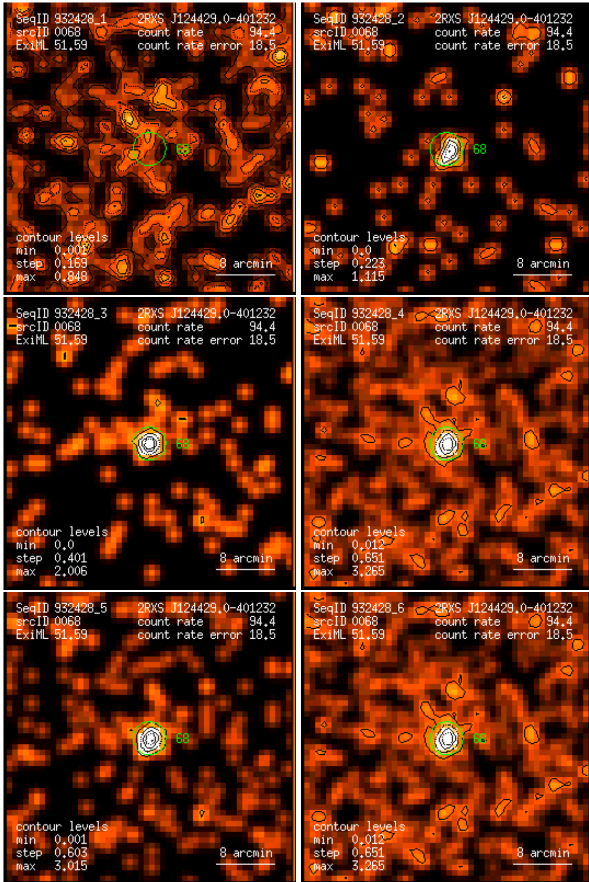
Figure 68: RASS 932428: detection 0068: band rate images, Gaussian filter: (1) PSPC channels 11 – 41, (2) 52 – 90, (3) 91 – 201, (4) 11 – 235, (5) 52 – 201, (6) 11 – 201. Broad band rates in counts/ks. Band rate contour levels in counts/ks/arcmin 2 .
